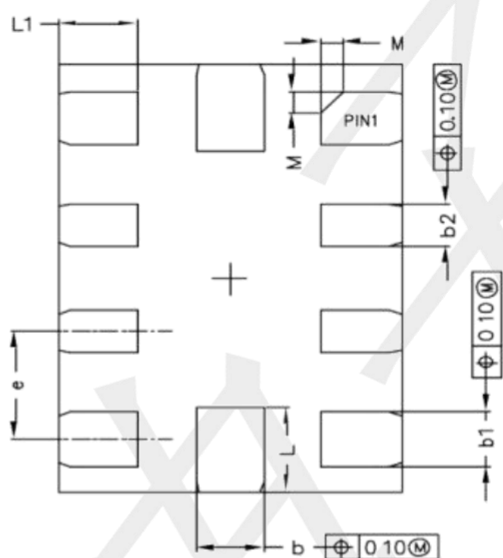
BOTTOM VIEW
