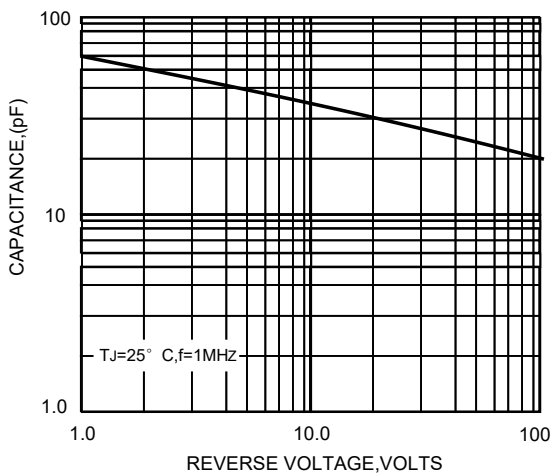
FIG.3-TYPICAL JUNCTION CAPACITANCE
