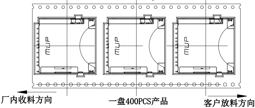
Carrier Dimensions Diagram: Pull out direction
