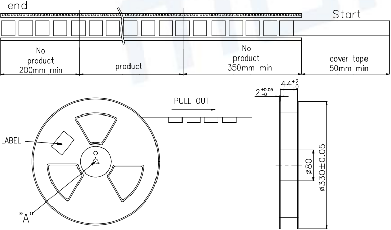
Reel Form Diagram:
