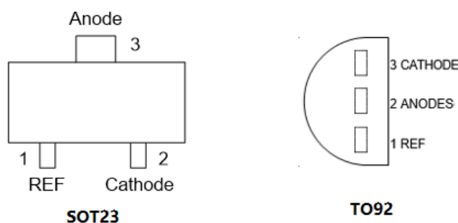
Figure 1. Package types of uP431H
