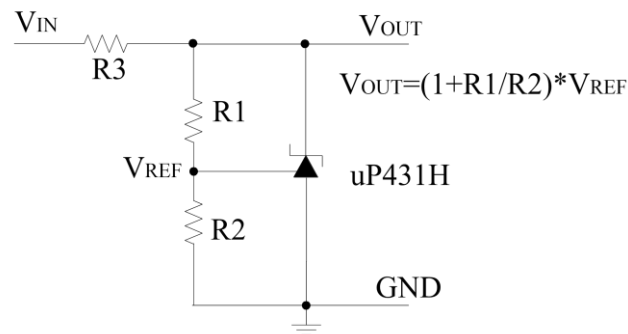
Shunt Regulator
