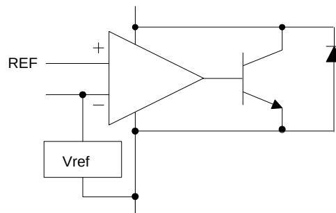
Figure 2. Functional Block Diagram of uP431H
