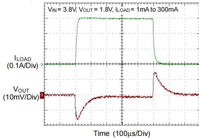
Load Transient
