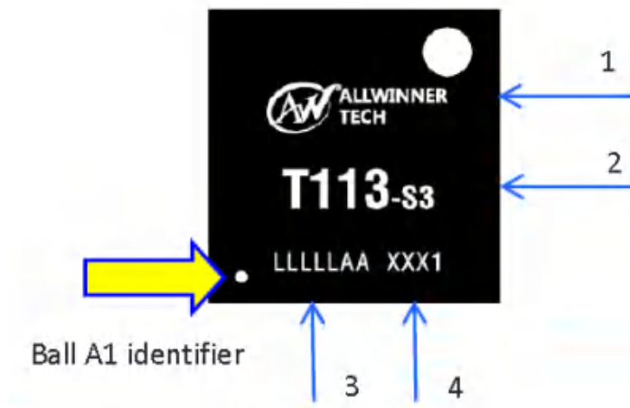
Figure 11-1 T113-S3 Marking
