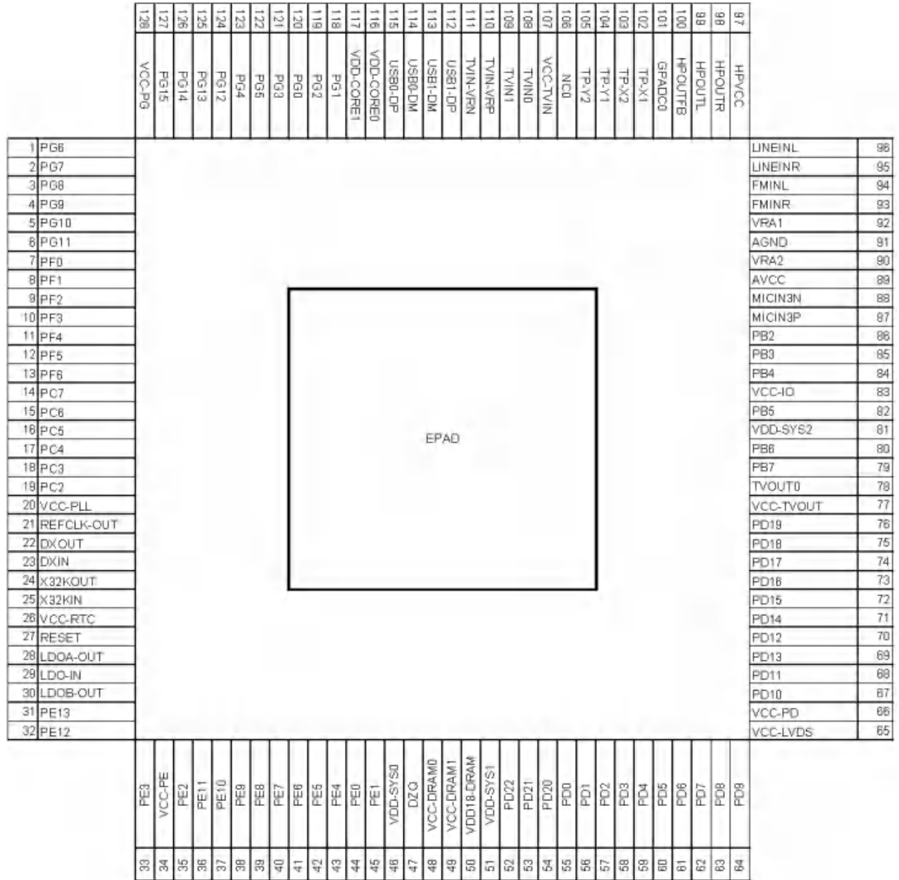
Figure 7-1 T113-S3 Pin Map
