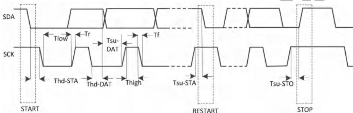
Figure 5-22 TWI Timing
