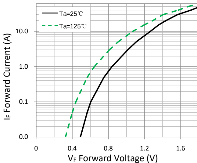
Figure 1. Forward Characteristic(typ.)
