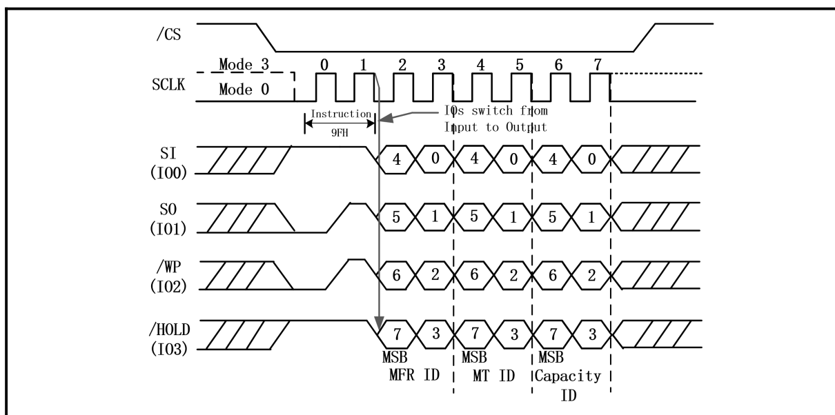
Figure 42. JEDEC ID Sequence Diagram (QPI Mode)
