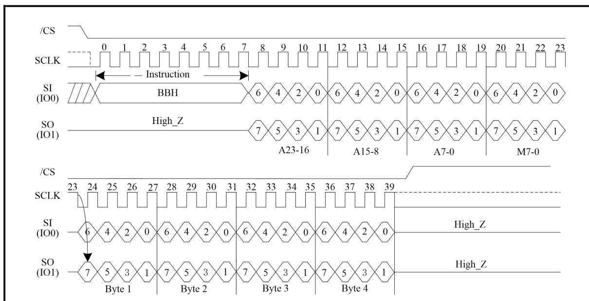
Figure 26. Dual I/O Fast Read Sequence Diagram (Initial instruction or previous (M5-4) ≠ (1,0) , SPI Mode only)
