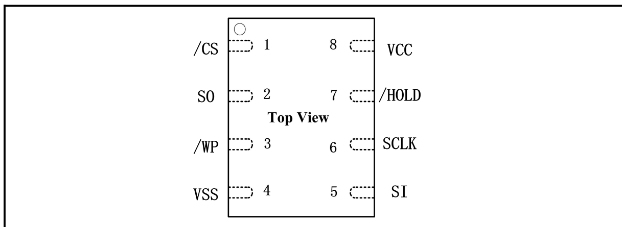
Figure 3. Pin Configuration USON8 2*3mm, WSON8 5*6mm and WSON8 6*8mm
