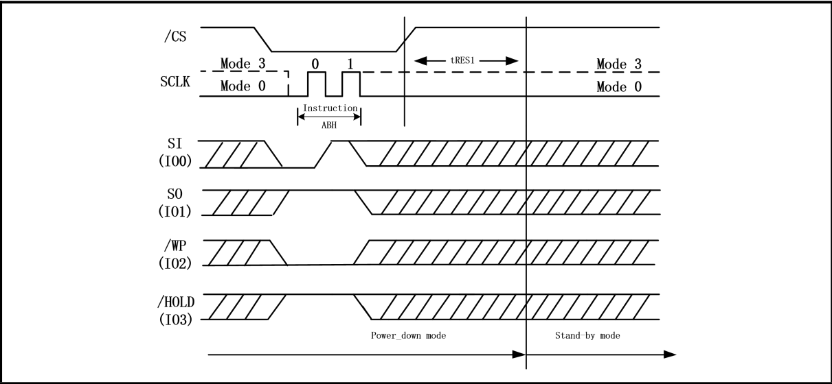
Figure 57. Release Power-Down/Read Device ID Sequence Diagram (SPI Mode)
