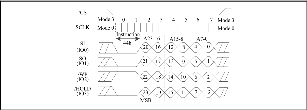
Figure 62. Erase Security Registers instruction Sequence Diagram (QPI Mode)
