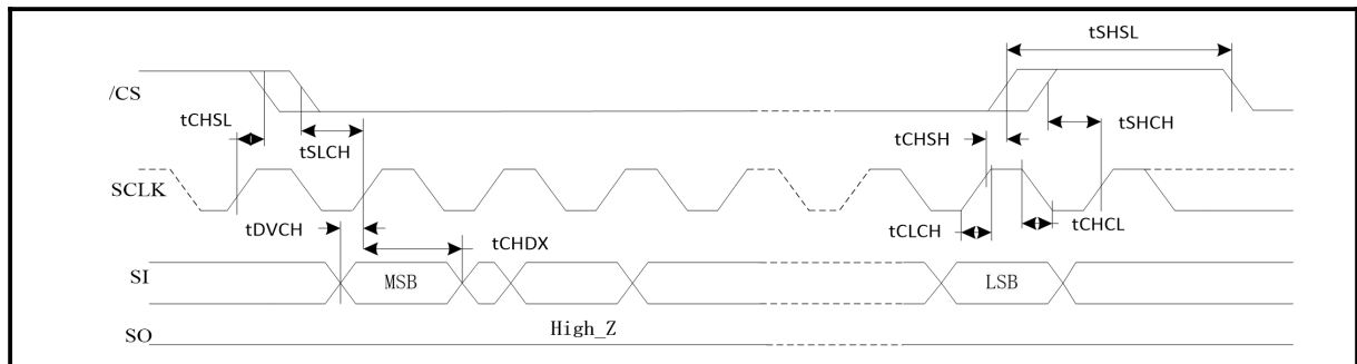
Figure 85. Output Timing
