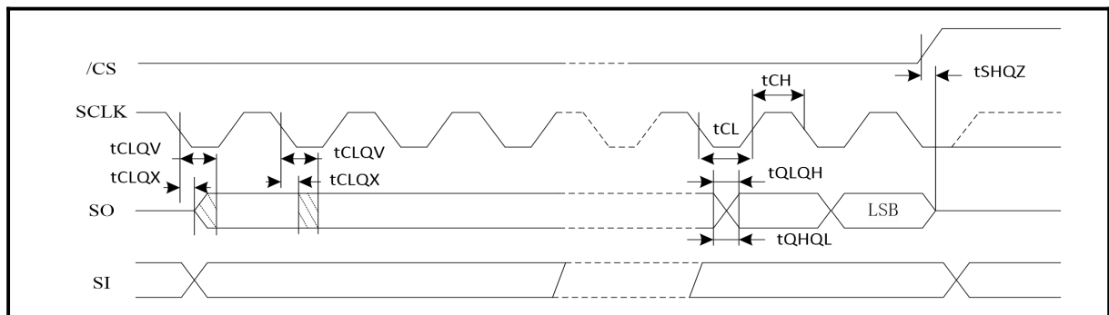
Figure 86. Hold Timing
