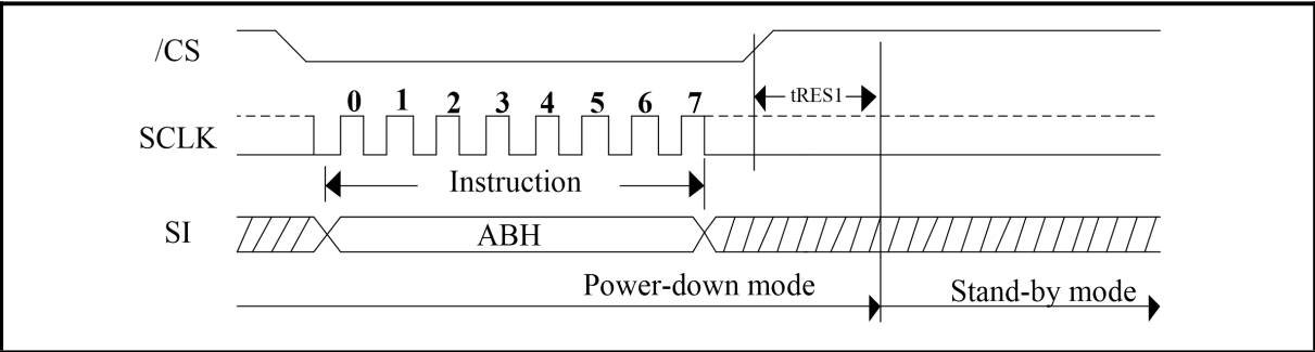
Figure 55. Release Power-Down Sequence Diagram (SPI Mode)
