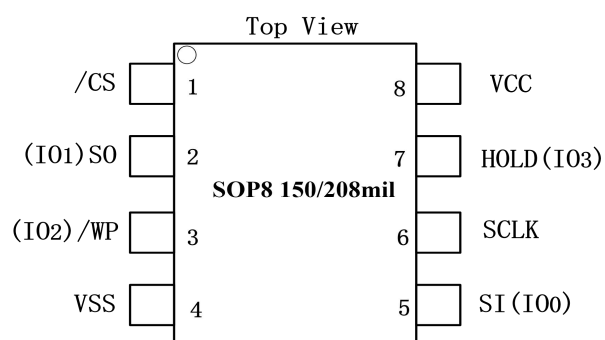
Figure 2. Pin Configuration SOP8 150mil/208mil
