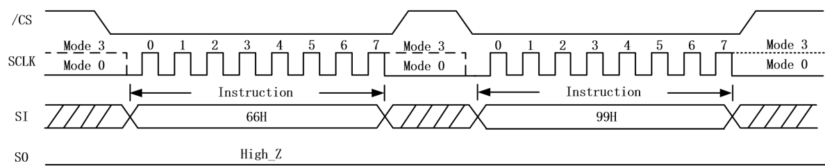
Figure 7.4.14. Enable Reset and Reset Instruction Sequence
