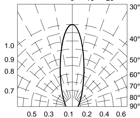
Fig.6-Radiation Diagram
