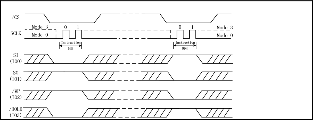
Figure 21. Enable Reset (66h) and Reset (99h) Instruction Sequence (QPI Mode)
