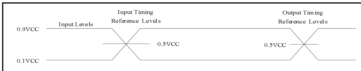
Figure 74. AC Measurement I/O Waveform
