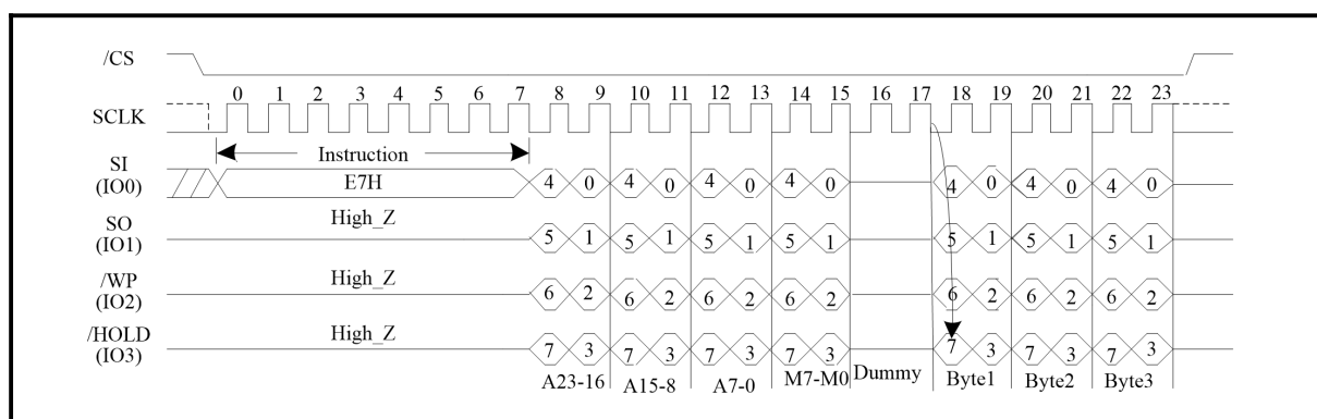
Figure 34. Quad I/O Word Fast Read Sequence Diagram (SPI Mode; Initial instruction or previous (M5-4)=(1,0))
