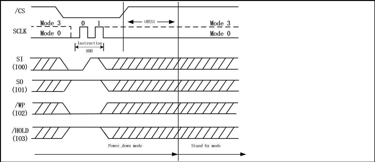
Figure 49. Release Power-Down/Read Device ID Sequence Diagram (SPI Mode)
