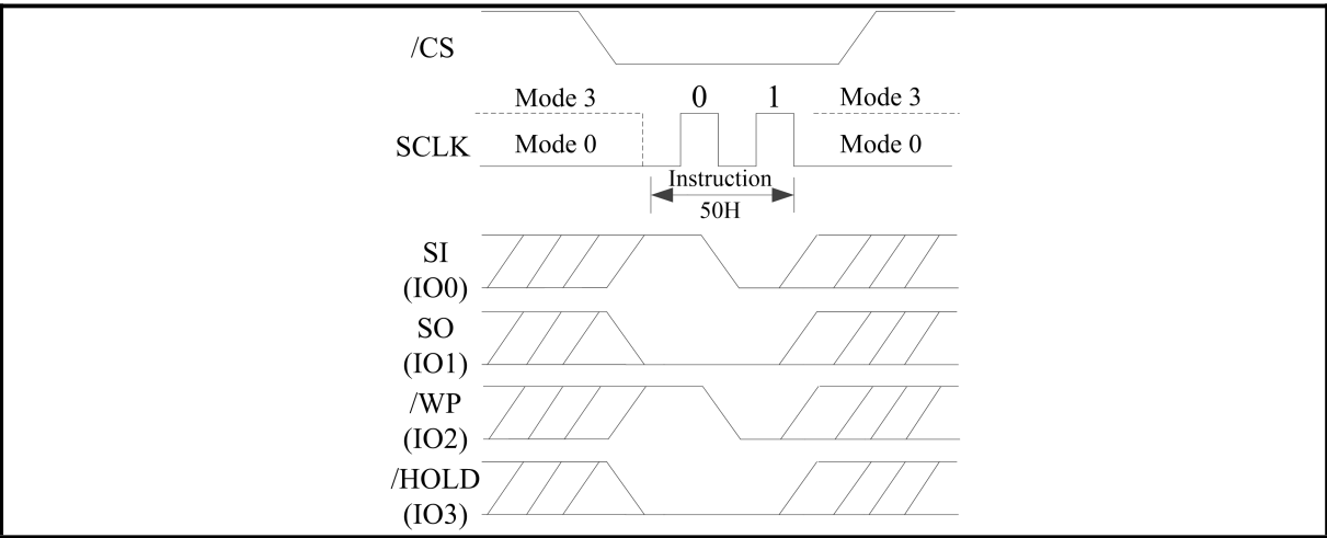
Figure 9. Write Enable for Volatile Status Register (QPI Mode)
