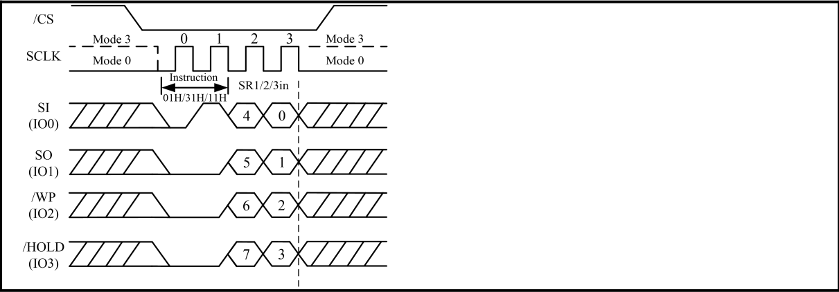
Figure 17. Write Status Register Sequence Diagram-01/31/11H 1byte (QPI Mode)
