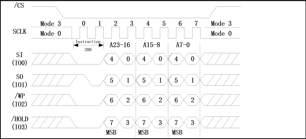
Figure 63. Sector Erase Sequence Diagram (QPI Mode/3-Byte Address Mode)
