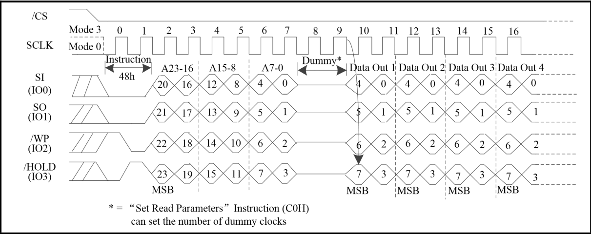
Figure 52. Read Security Registers instruction Sequence Diagram (QPI Mode)
