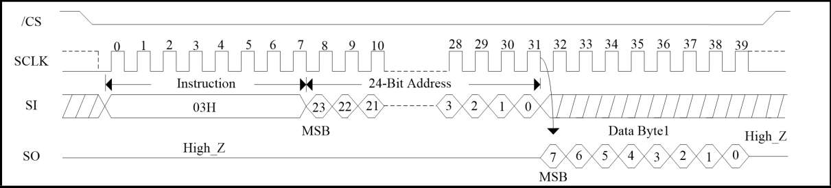
Figure 22. Read Data Bytes Sequence Diagram (SPI Mode only)
