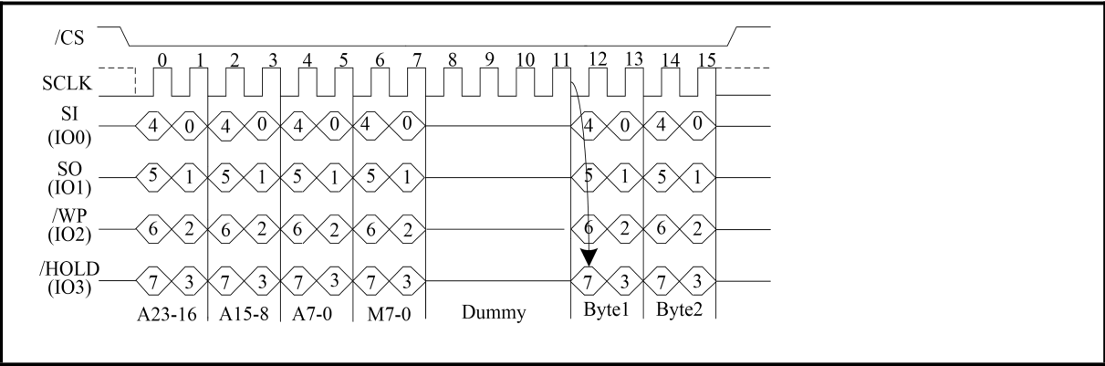
Figure 32. Quad I/O Fast Read Sequence Diagram (QPI Mode Mode; Initial instruction or previous (M5-4=(1,0)))
