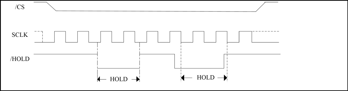
Figure 5. Hold condition activation
