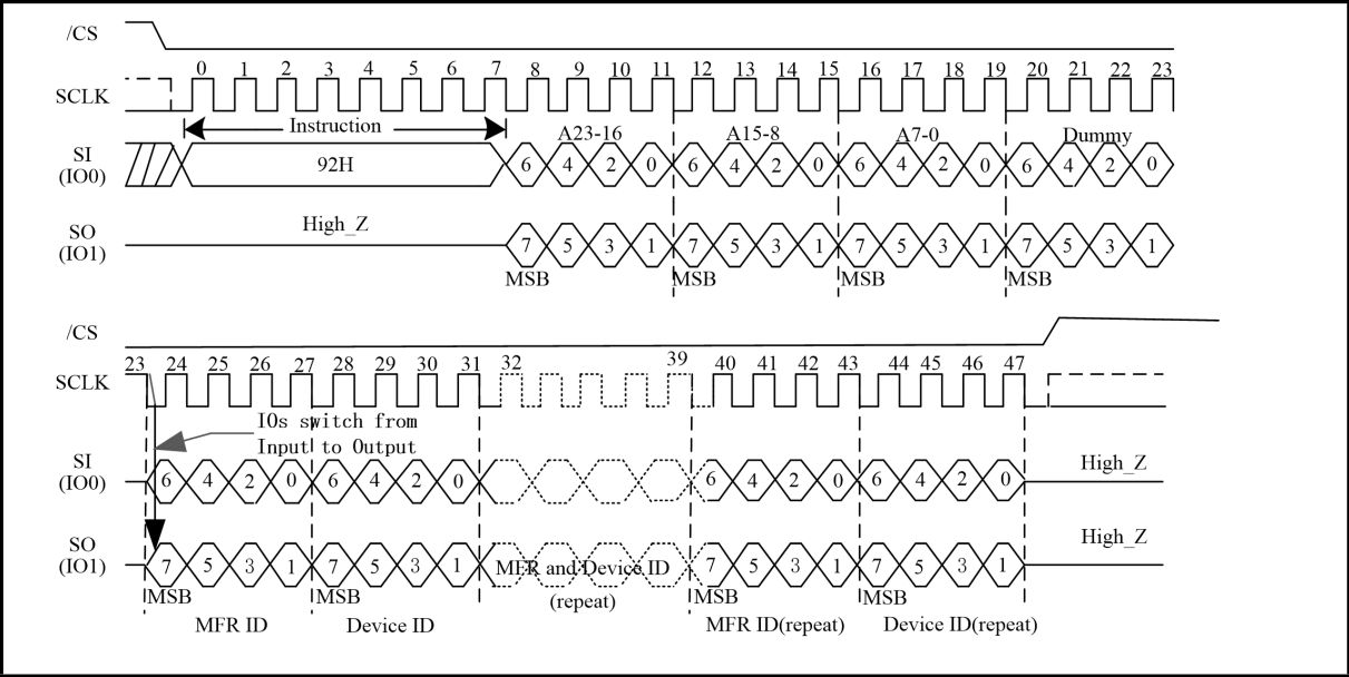
Figure 40. Dual I/O Read Manufacture ID/ Device ID Sequence Diagram (SPI Mode)
