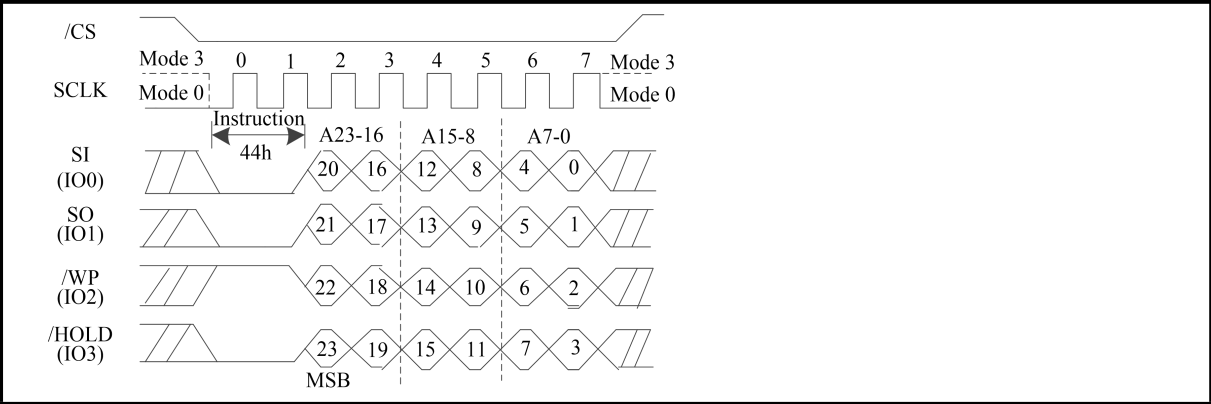
Figure 54. Erase Security Registers instruction Sequence Diagram (QPI Mode)
