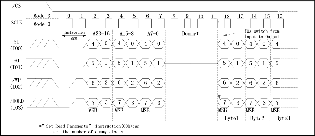
Figure 37. Burst Read with Wrap (QPI Mode only)
