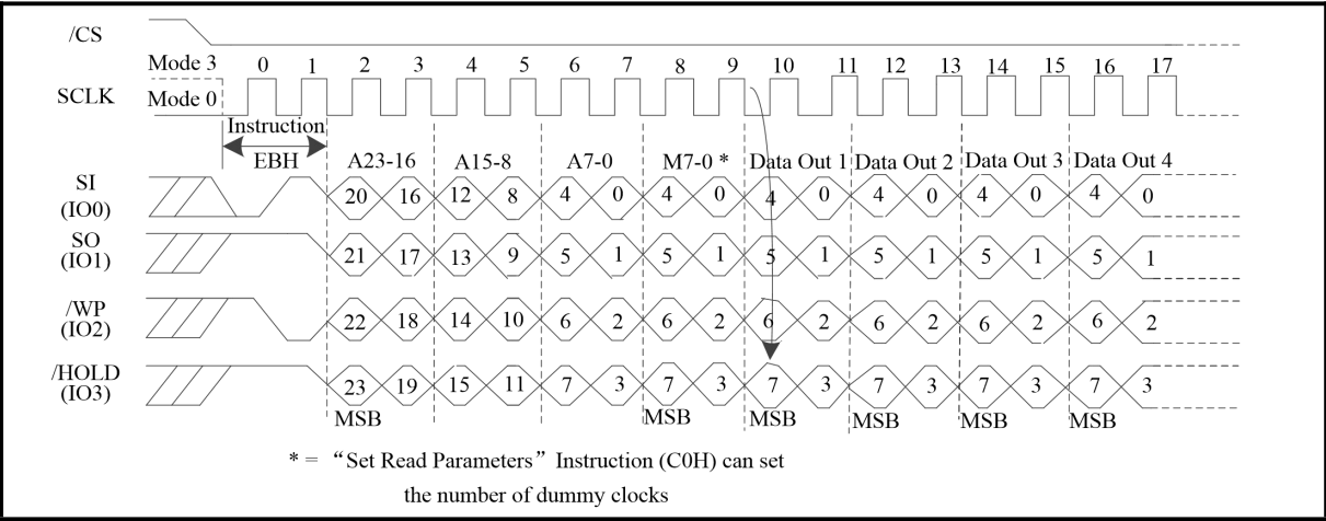
Figure 31. Quad I/O Fast Read Sequence Diagram (QPI Mode Mode; Initial instruction or previous (M5-4≠(1,0)))
