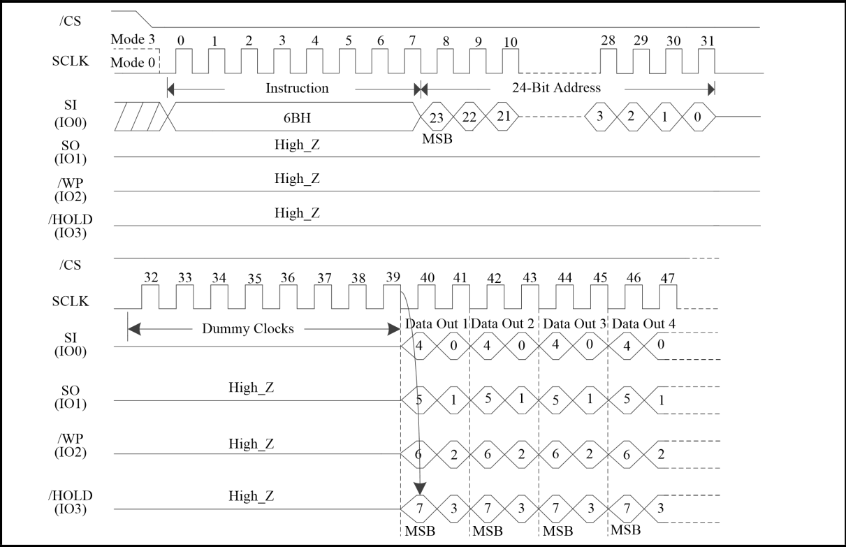
Figure 26. Quad Output Fast Read Sequence Diagram (SPI Mode only)
