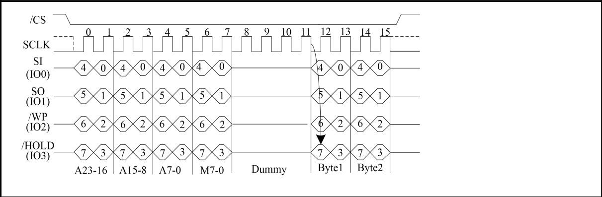
Figure 30. Quad I/O Fast Read Sequence Diagram (SPI Mode; Initial instruction or previous (M5-4=(1,0)))
