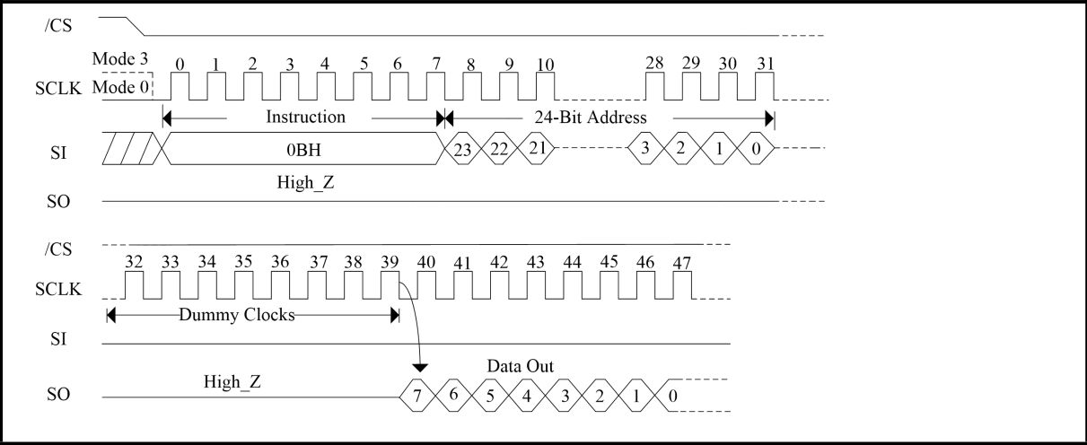
Figure 23. Fast Read Sequence Diagram (SPI Mode)
