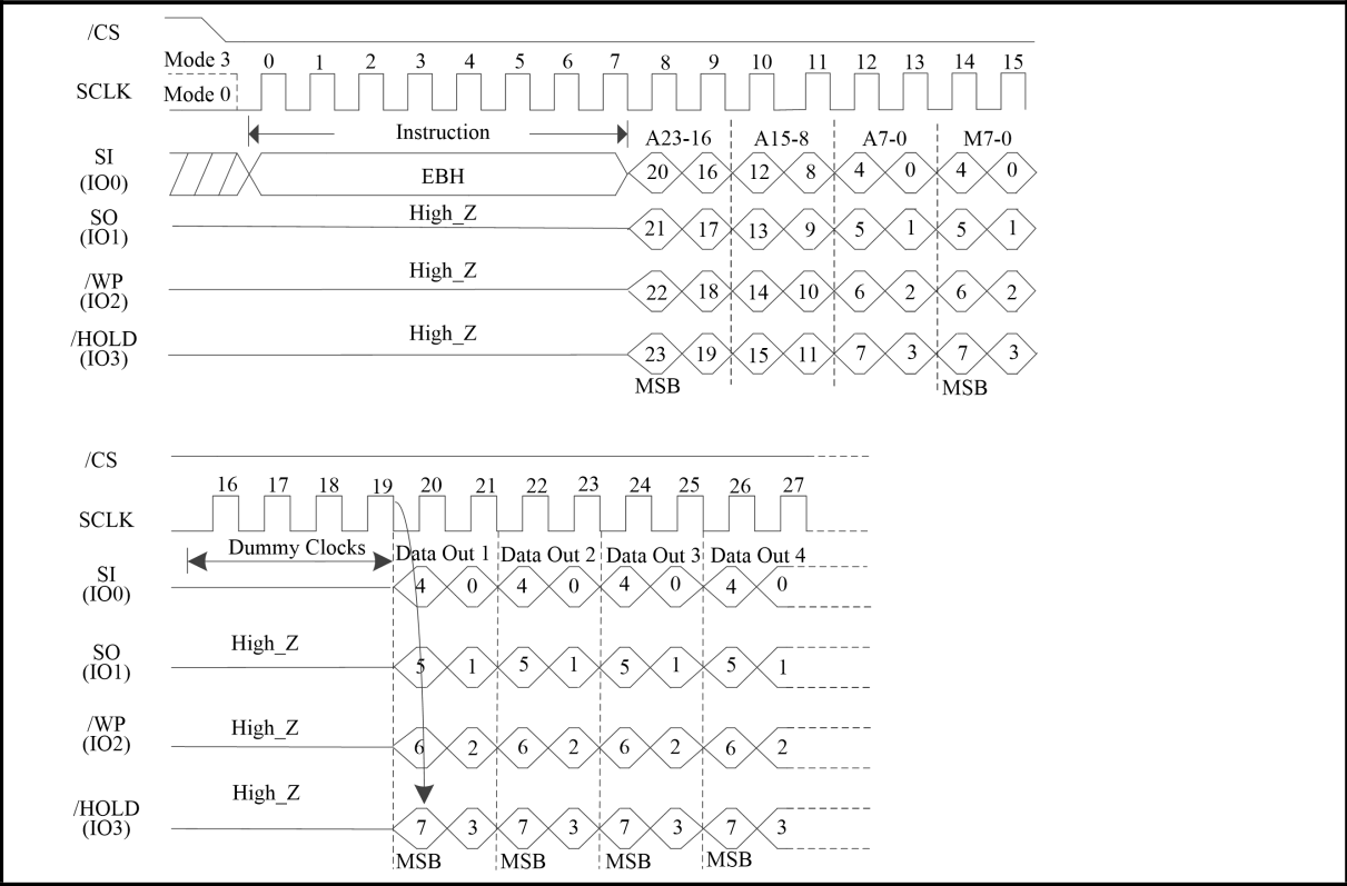
Figure 30. Quad I/O Fast Read Sequence Diagram (SPI Mode; Initial instruction or previous (M5-4=(1,0)))
