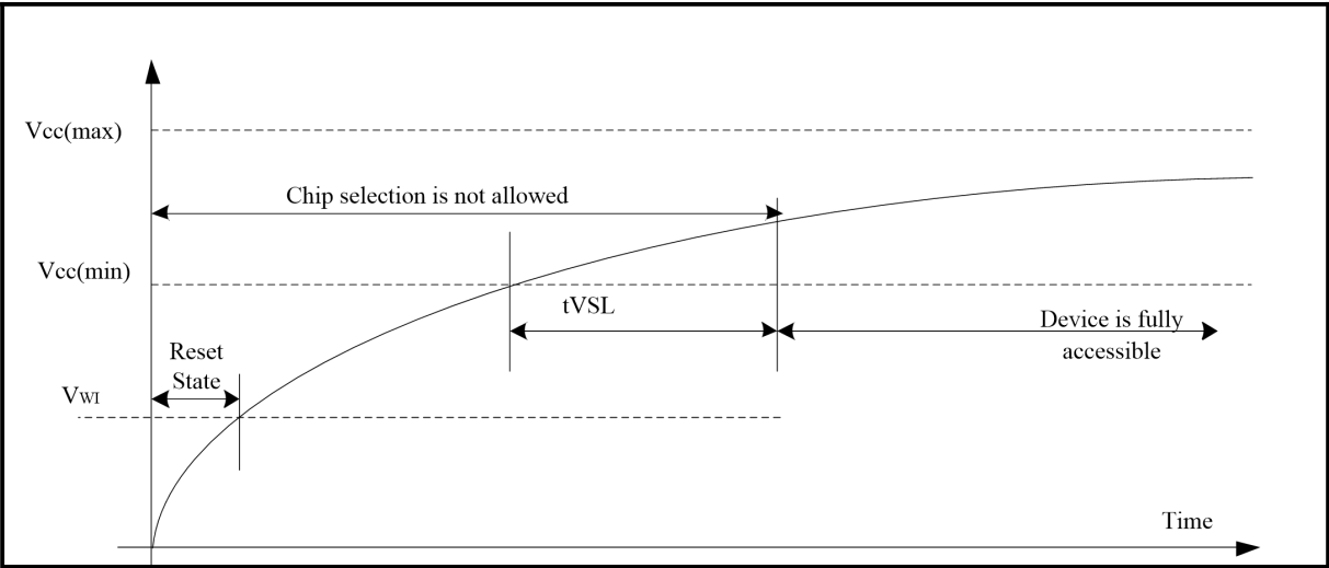
Figure 73. Power-up Timing and Voltage Levels
