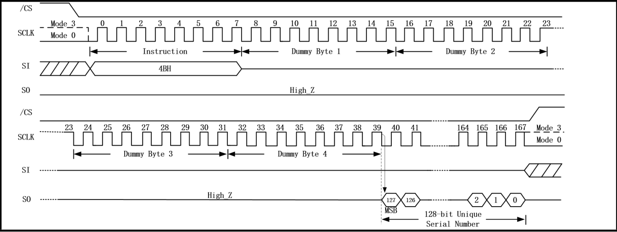
Figure 44. Read Unique ID Sequence Diagram (SPI Mode only)
