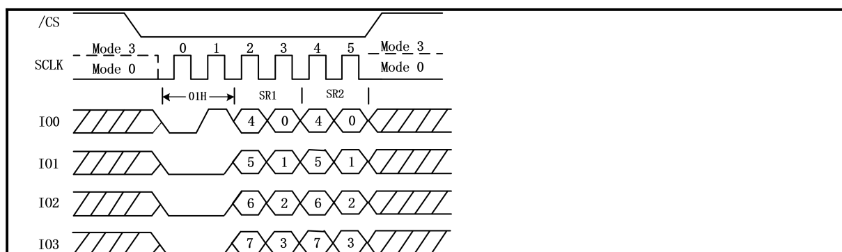
Figure 15. Write Status Register Sequence Diagram-01H 2byte (QPI Mode)
