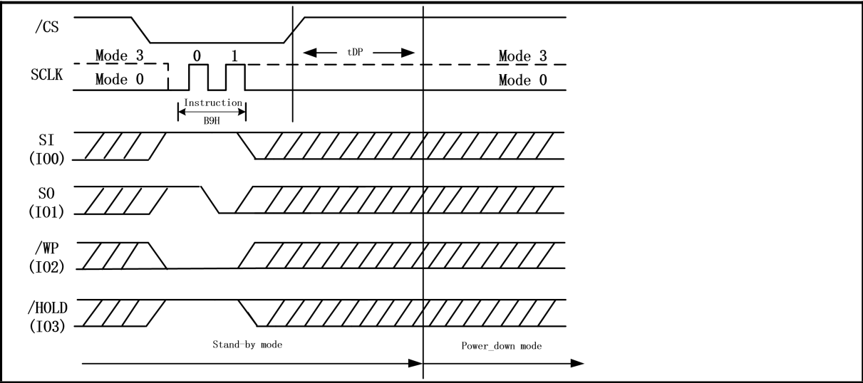
Figure 46. Deep Power-Down Sequence Diagram (QPI Mode)
