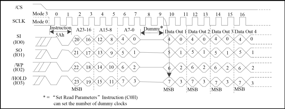
Figure 58. Read Serial Flash Discoverable Parameter instruction Sequence Diagram (QPI Mode)
