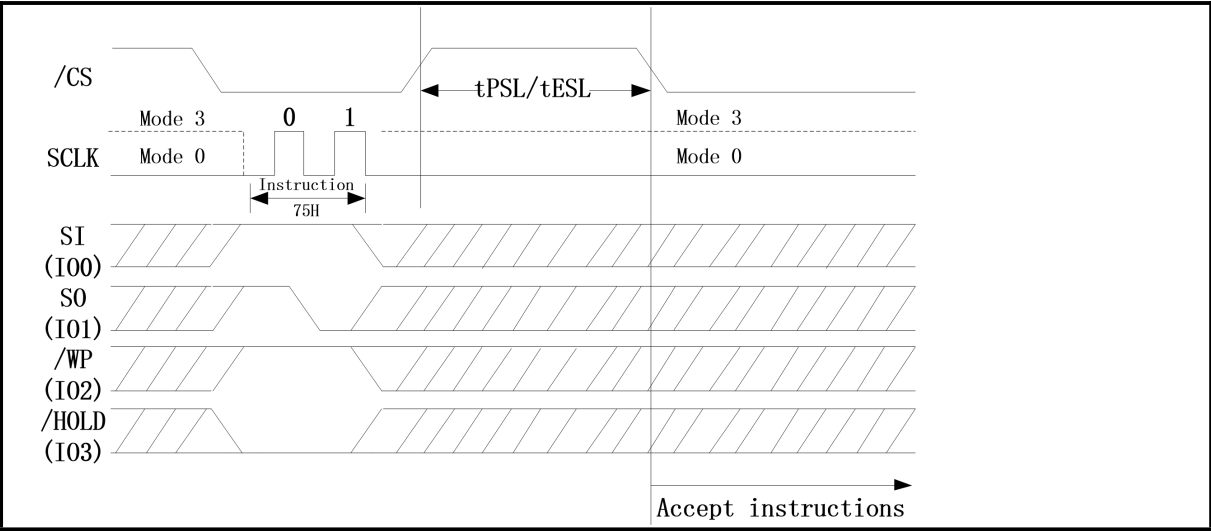
Figure 71. Program/Erase Suspend Instruction Sequence (QPI Mode)
