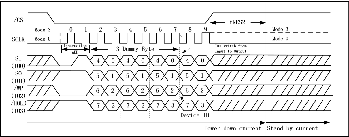
Figure 50. Release Power-Down/Read Device ID Sequence Diagram (QPI Mode)
