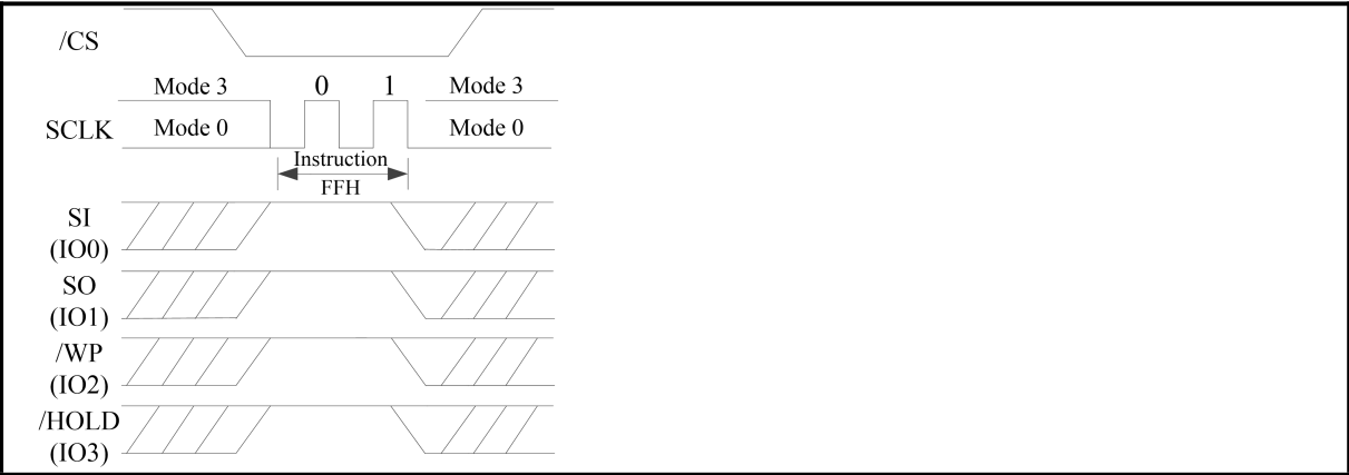
Figure 19. Exit QPI Mode (QPI Mode)
