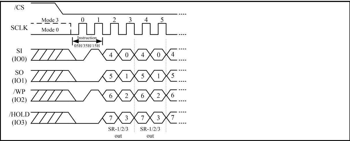
Figure 13. Read Status Register Sequence Diagram (QPI Mode)
