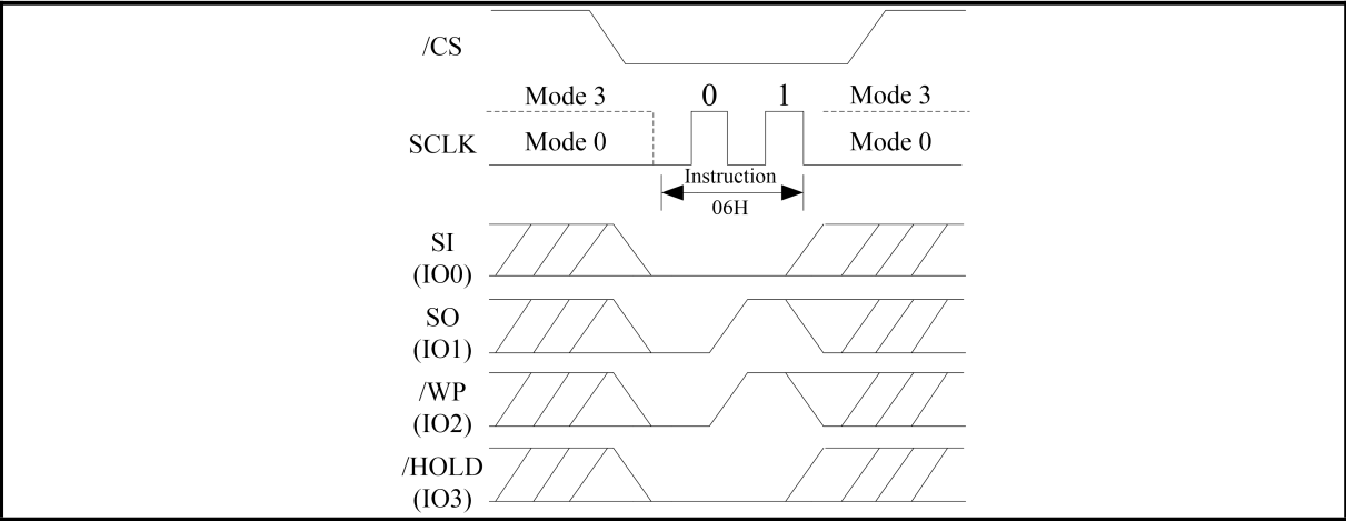
Figure 7. Write Enable Sequence Diagram (QPI Mode)
