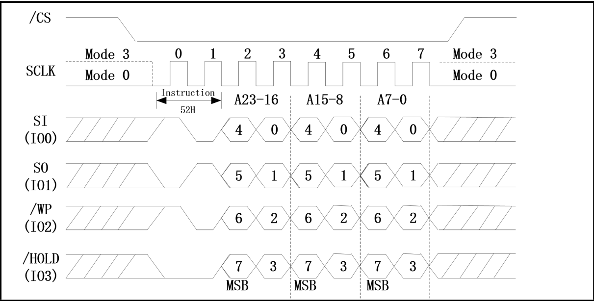
Figure 65. 32KB Block Erase Sequence Diagram (QPI Mode)
