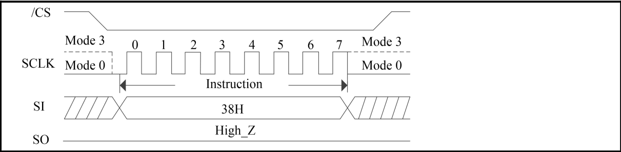
Figure 18. Enter QPI Mode (SPI Mode)
