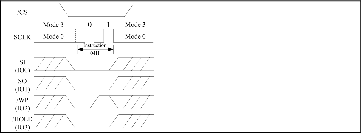
Figure 11. Write Disable Sequence Diagram (QPI Mode)
