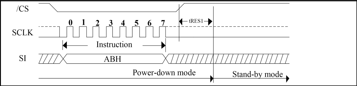
Figure 48. Release Power-Down Sequence Diagram (QPI Mode)
