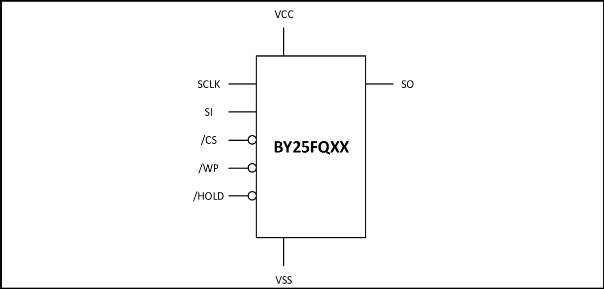
Figure 2. Pin Configuration SOP 150mil/208 mil
