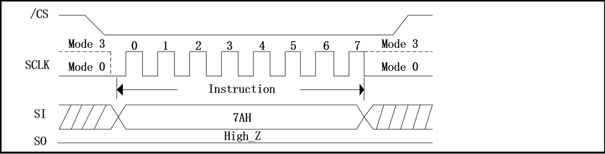
Figure 72. Program/Erase Resume Instruction Sequence (SPI Mode)
