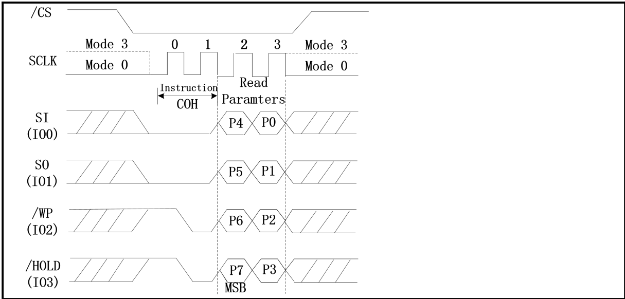
Figure 36. Burst Read with Wrap (QPI Mode only)
