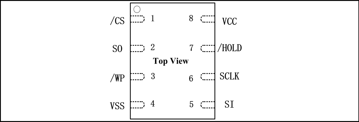
Figure 3. Pin Configuration USON8 2*3mm(0.55mm), WSON8 5*6mm
