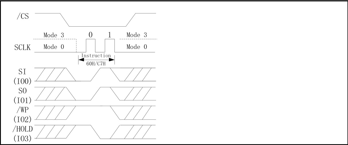
Figure 69. Chip Erase Sequence Diagram (QPI Mode)
