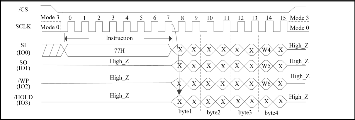
Figure 35. Set Burst with Wrap Sequence Diagram (SPI Mode only)
