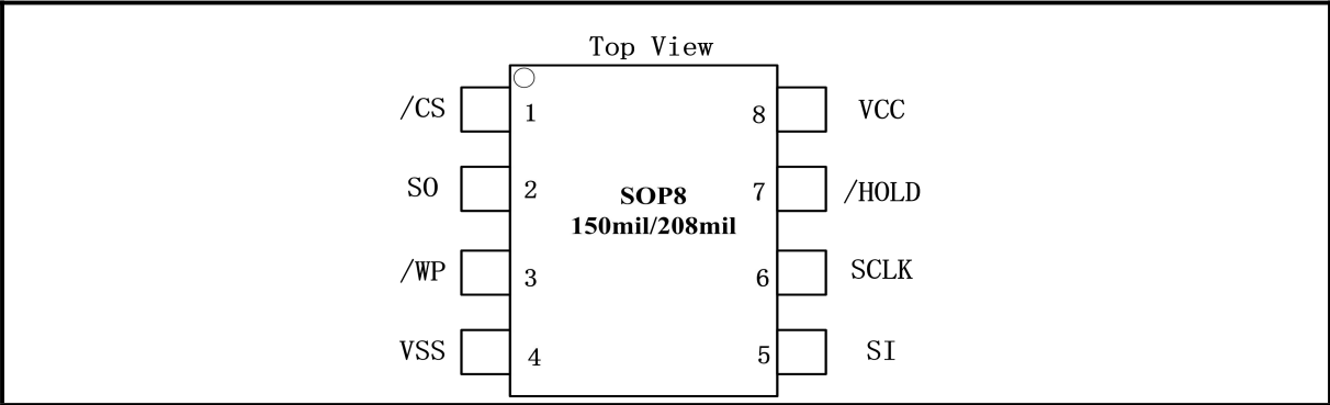
Figure 2. Pin Configuration SOP 150mil/208 mil
