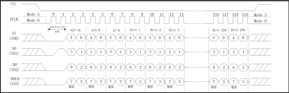
Figure 60. Page Program Sequence Diagram (QPI Mode)
