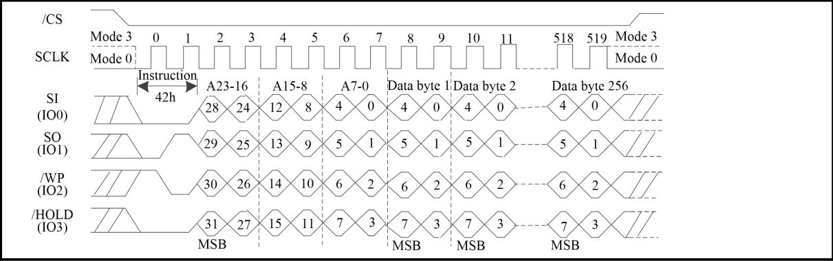
Figure 56. Program Security Registers instruction Sequence Diagram (QPI Mode)
