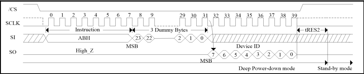
Figure 49. Release Power-Down/Read Device ID Sequence Diagram (SPI Mode)
