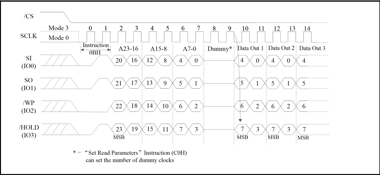
Figure 24. Fast Read Sequence Diagram (QPI Mode Mode)
