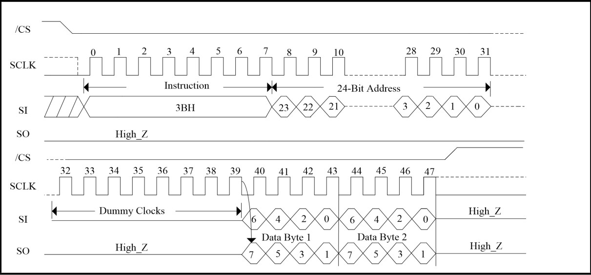
Figure 25. Dual Output Fast Read Sequence Diagram (SPI Mode only)
