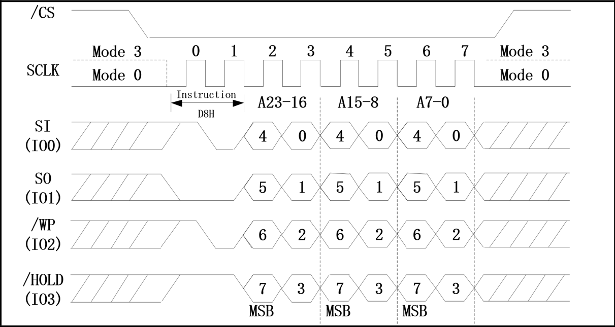
Figure 67. 64KB Block Erase Sequence Diagram (QPI Mode)
