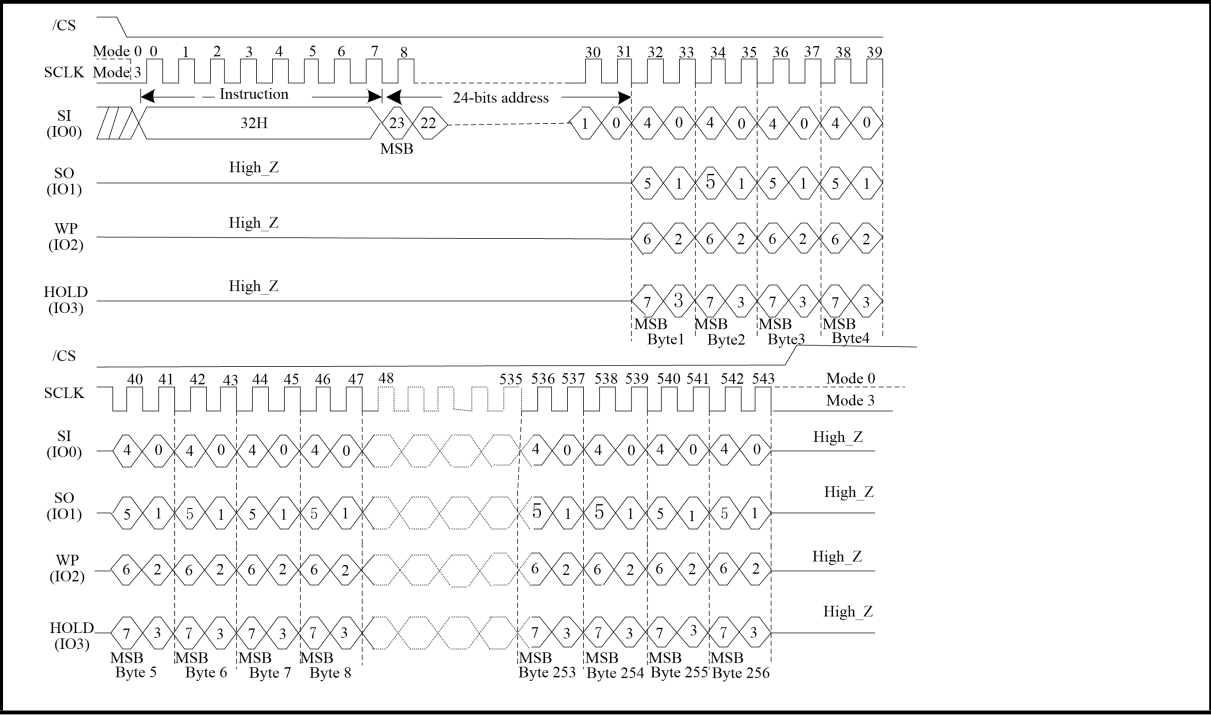
Figure 61. Quad Page Program Sequence Diagram (SPI Mode only)
