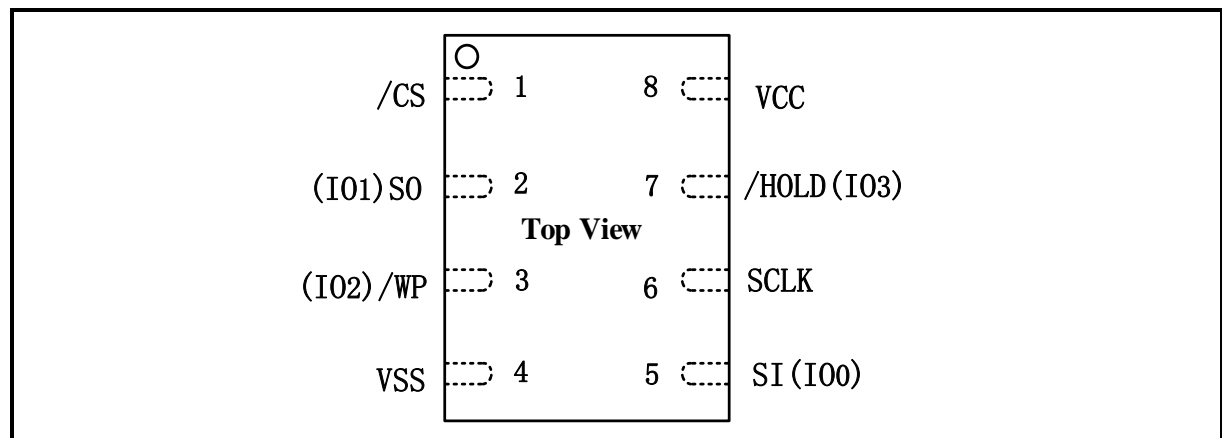
Figure 3. Pin Configuration WSON8 5*6mm,USON8 4*3mm and LGA8 2*3mm
