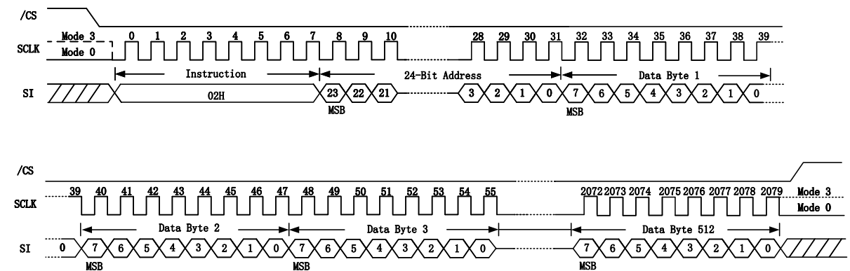
Figure 7.4.1. Page Program Instruction
