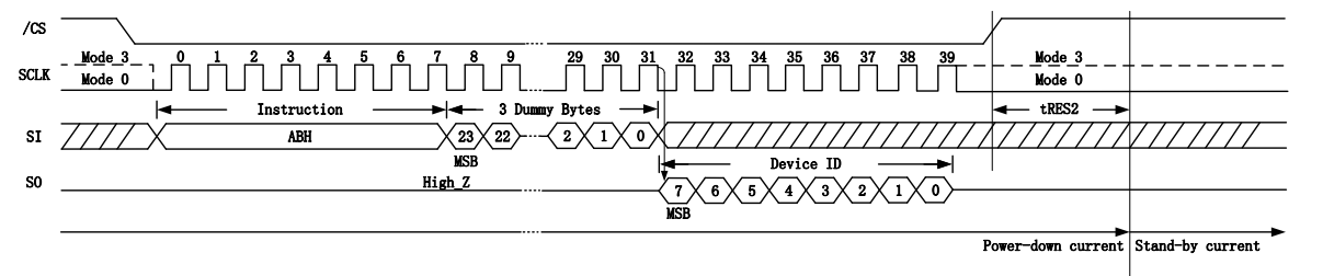
Figure 7.3.2b. Release Power-down / Device ID Instruction
