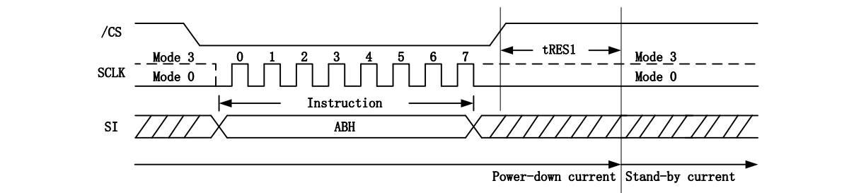
Figure 7.3.2b. Release Power-down / Device ID Instruction
