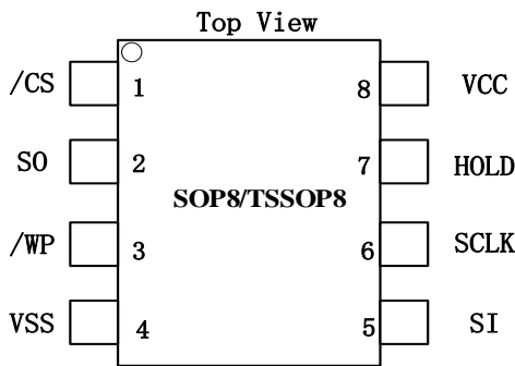
Figure 2. Pin Configuration SOP8/TSSOP8
