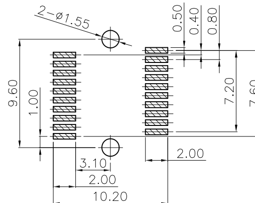
DETAIL A(SCALE 2:1)
