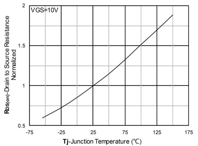
Normalized On-Resistance
