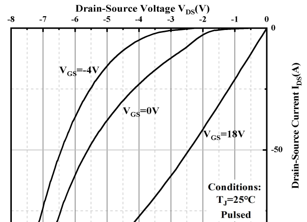
3rd Quadrant Characteristics( V_{GS}=18V )
