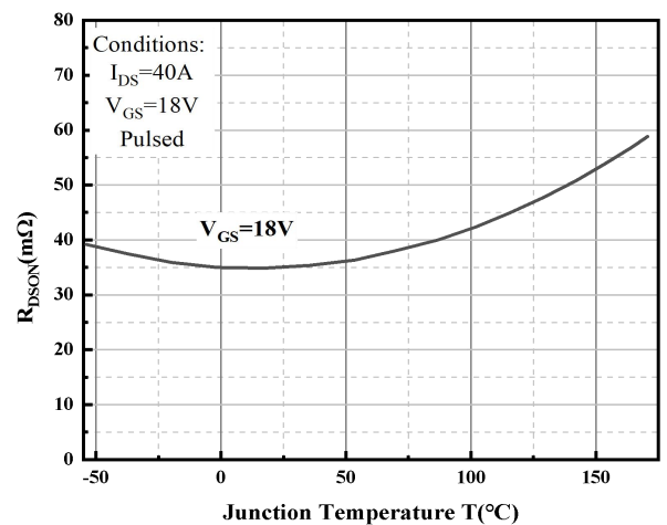
Typical On-Resistance characteristics
