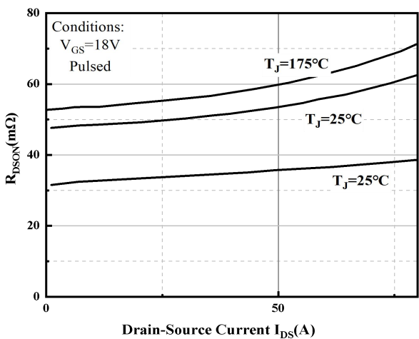
Typical On-Resistance characteristics
