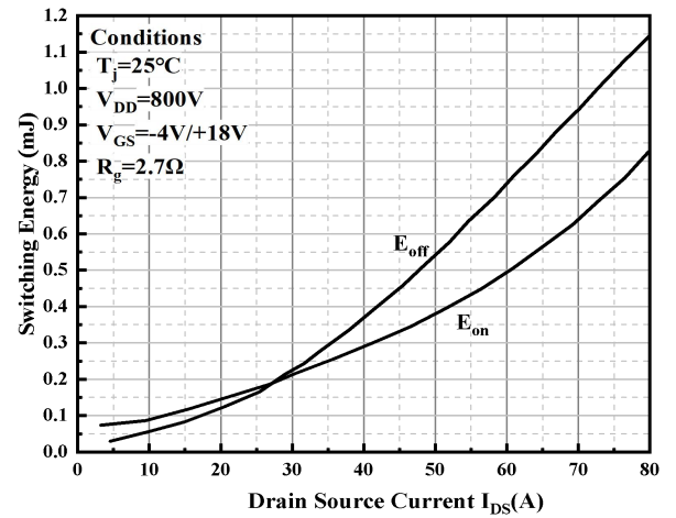
Typical MOSFET switching energy
