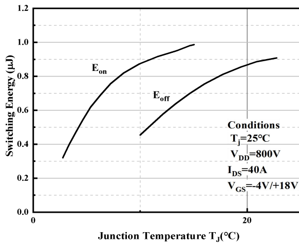
Typical MOSFET switching energy
