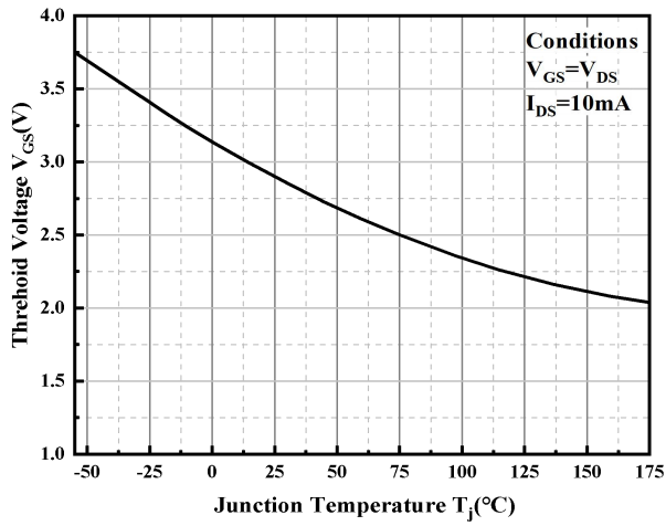
Typical V_{GS(th)} characteristics
