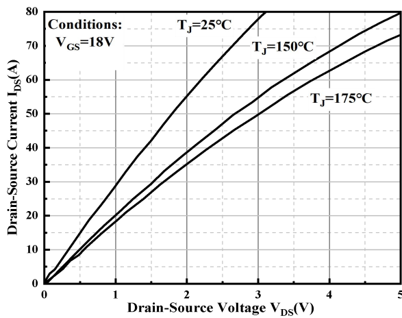
Typical output characteristic with different temperature
