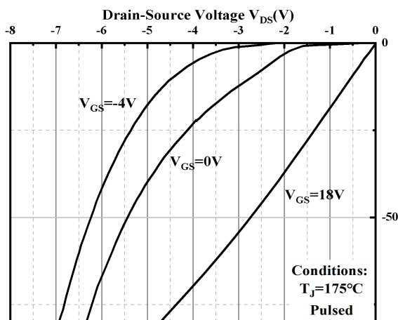
3rd Quadrant Characteristics( T_J = -40^\circ C )
