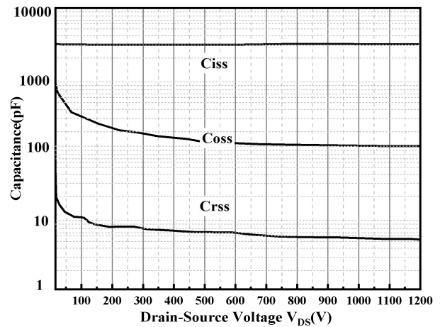
Typical capacity characteristic
