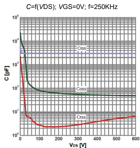
Figure 12: Typ. capacitances
