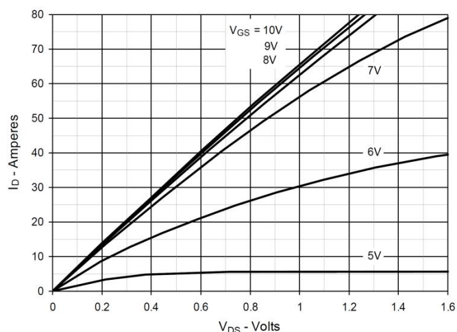
Output Characteristics
