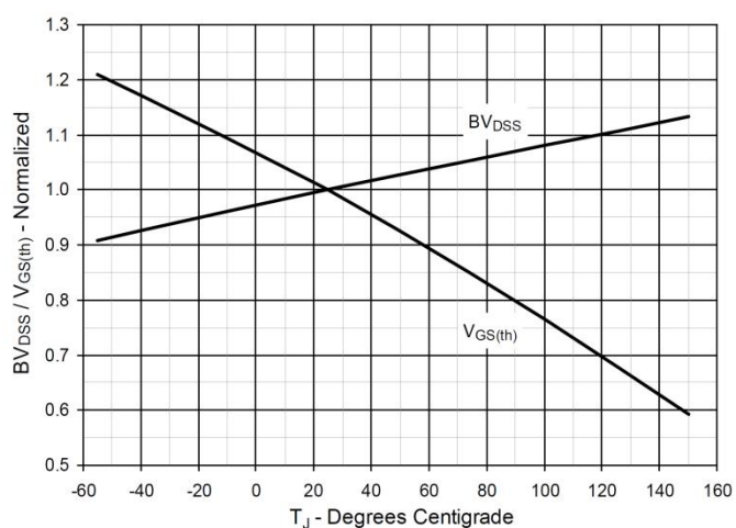
Normalized Breakdown & Threshold Voltages vs. Junction Temperature
