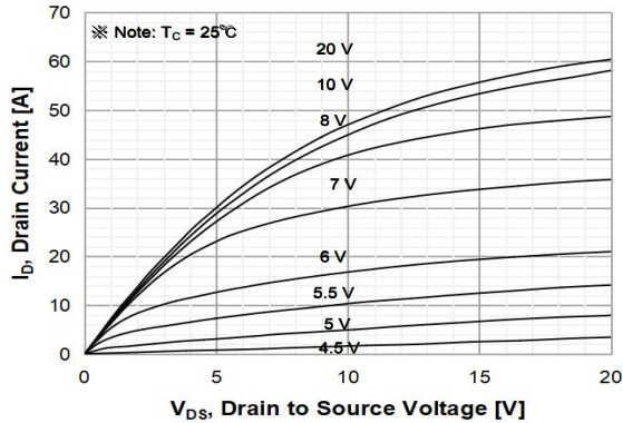
Figure 1. On-Region Characteristics
