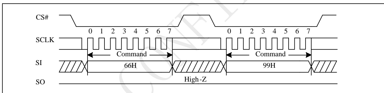
Figure 10-28a Reset Sequence
