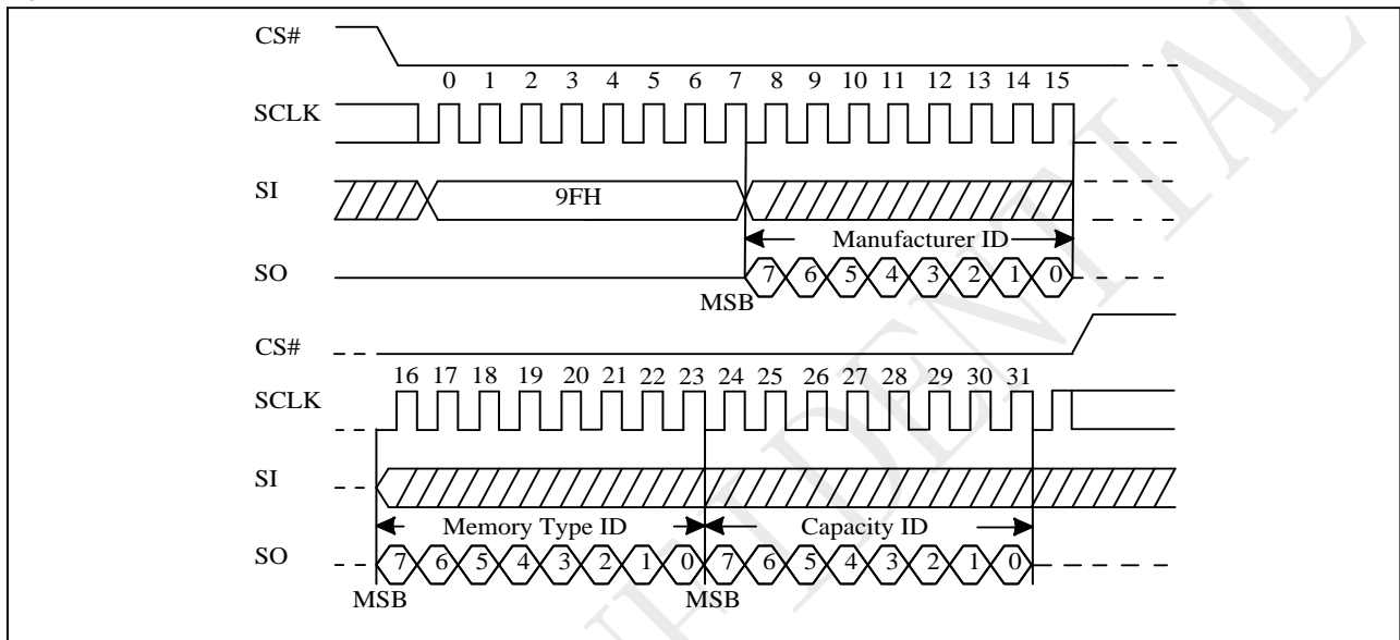
Figure 10-45 Read Identification (RDID) Sequence (Command 9F)
