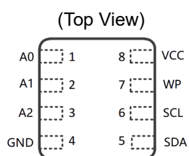
DFN-8 3*3
