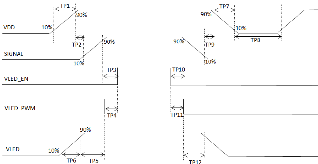
Figure 6.4 Interface power on/off sequence
