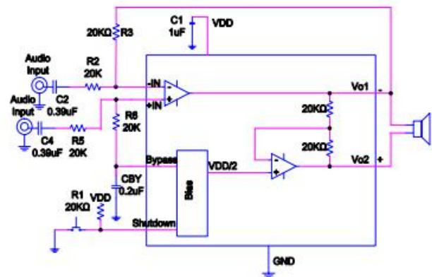
Figure 2.Differential Input
