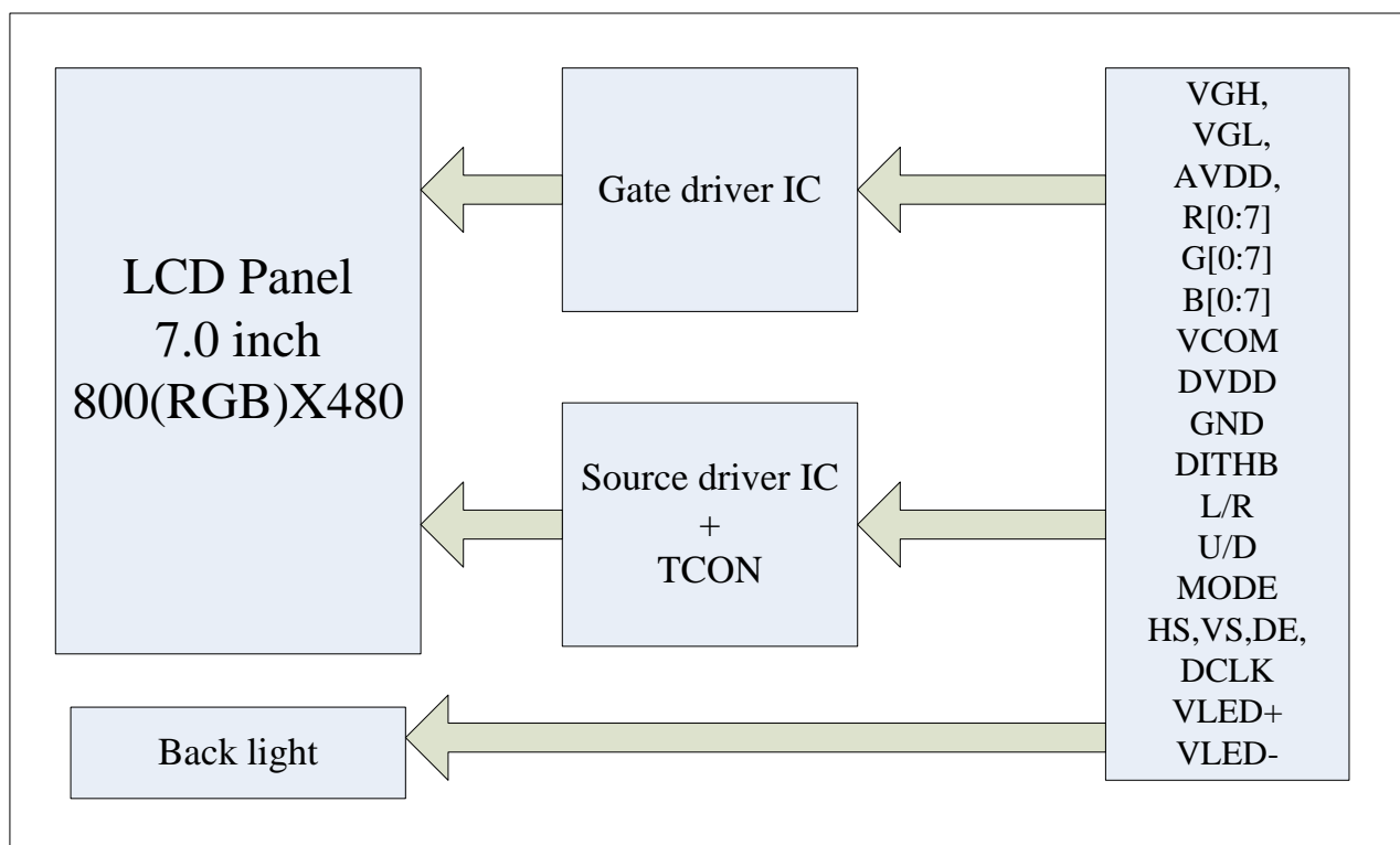
Figure 4.3 Block diagram
