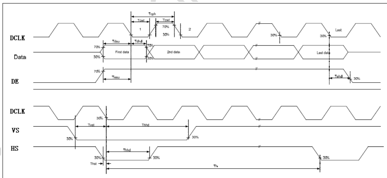
Figure 5.1 Input timing
