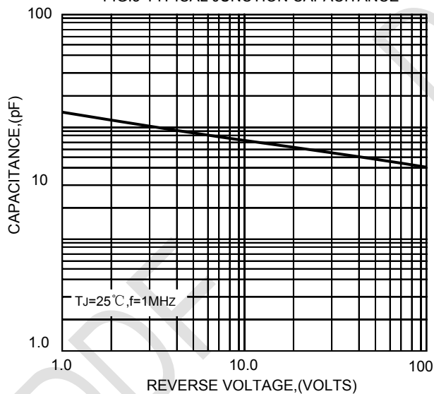
FIG.3-TYPICAL JUNCTION CAPACITANCE
