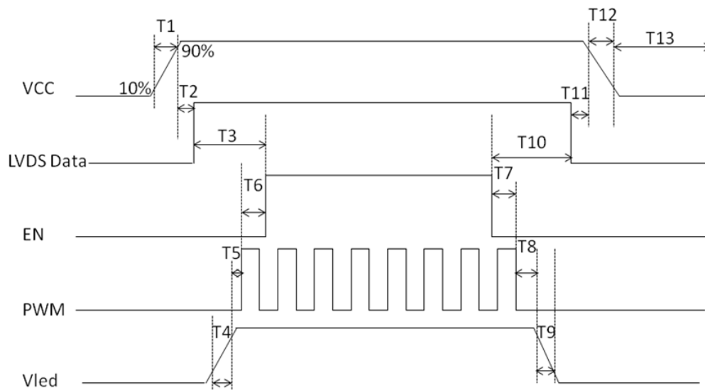
Figure 13 Power Sequence
