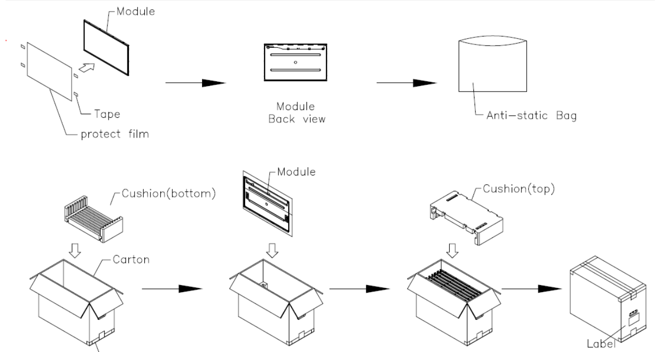
Figure. 9-1 Packing method
