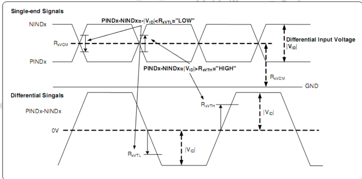
Figure 5.2 DC Electrical Characteristics
