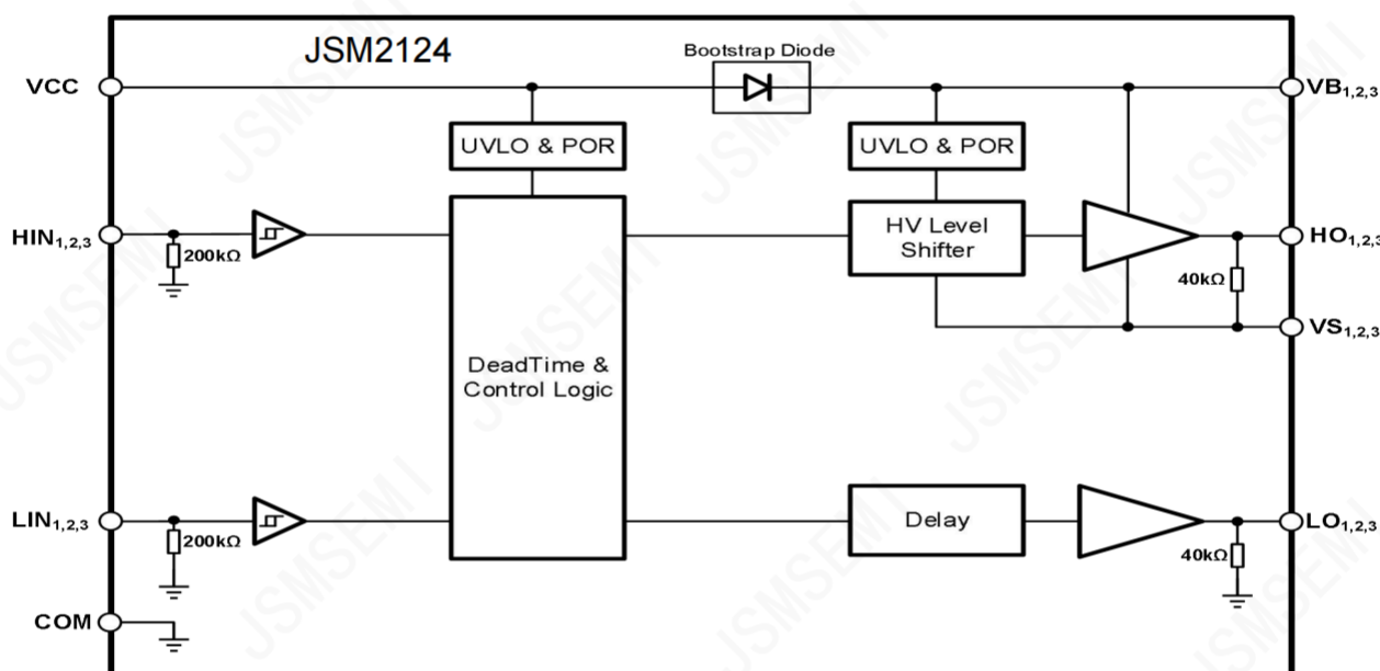
Figure7-1 Function Block Diagram of JSM2124
