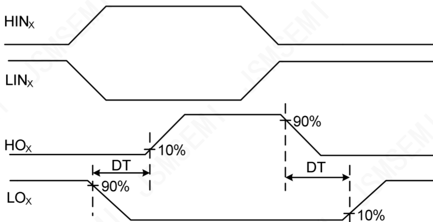
Input and output timing waveform Figure 6-
