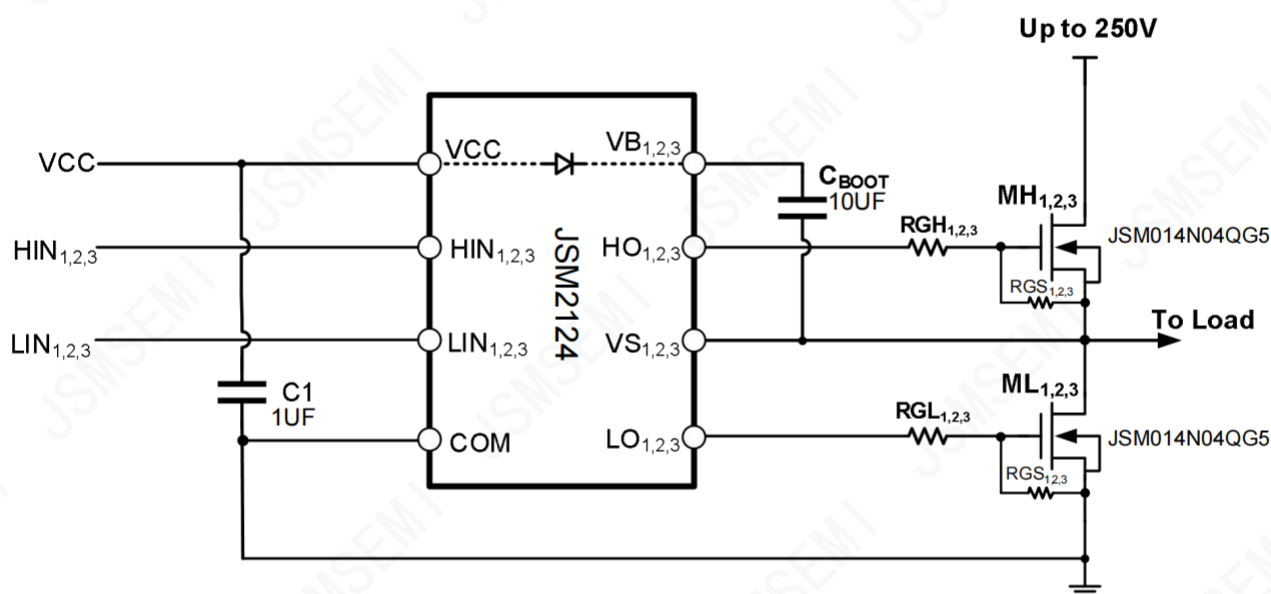
Figure 8-1 Typical application circuit of JSM2124
