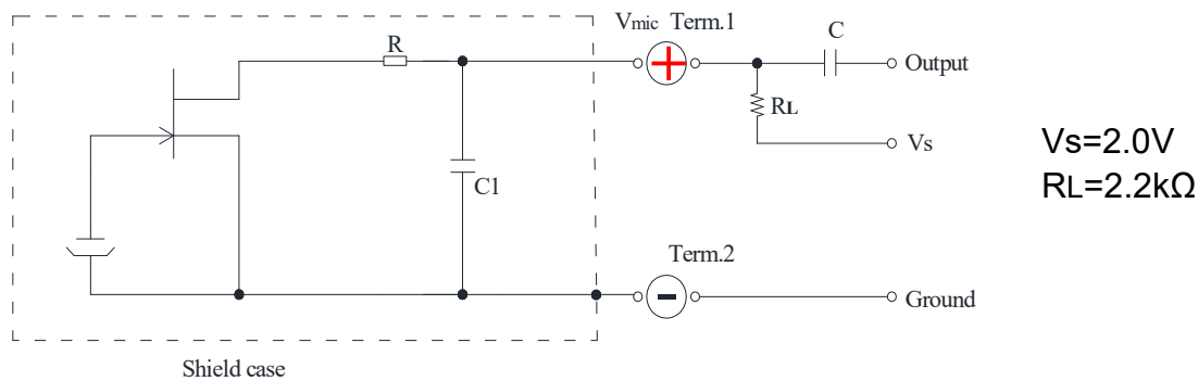
Fig. 5-1 Schematic Diagram
