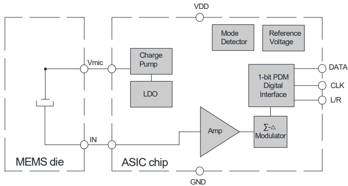
Fig. 1 Microphone block diagram
