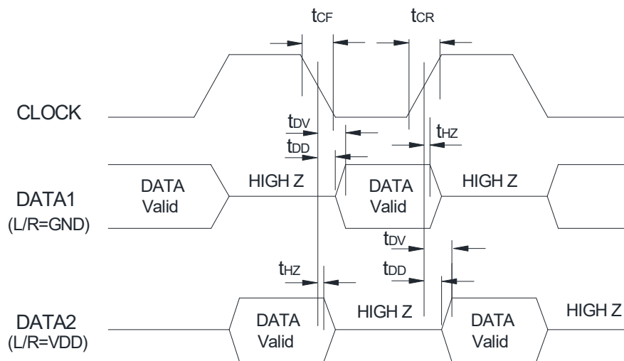
Fig. 2 Recommended timing diagram
