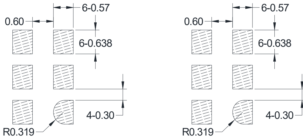
Example Land Pattern Example Solder Stencil Pattern
