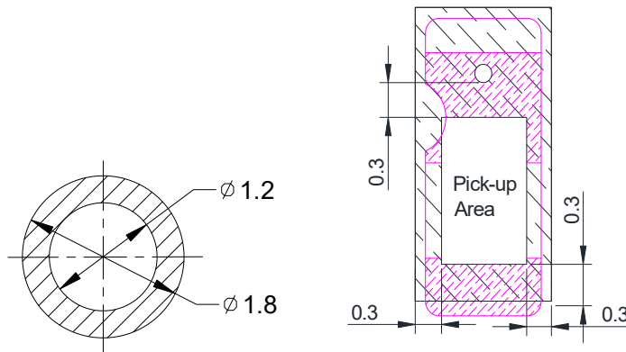
Fig. 15 Recommended nozzle for reflow MIC and Pick-up Area
