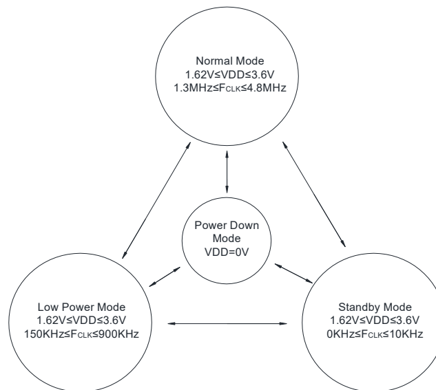
Fig. 3 State diagram
