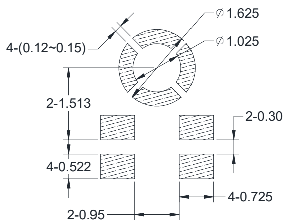
Example Solder Stencil Pattern
