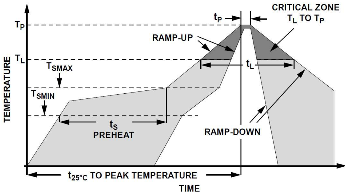
Fig. 13 Reflow Profile
