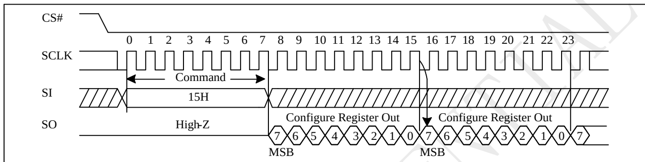
Configure Register
