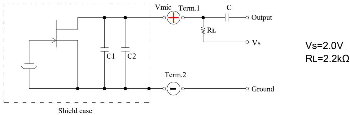
Fig. 5-1 Schematic Diagram
