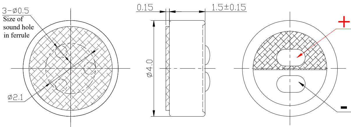
Fig. 7-1 Microphone capsule
