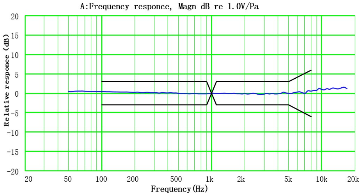
Fig. 4-1 Typical Frequency Response
