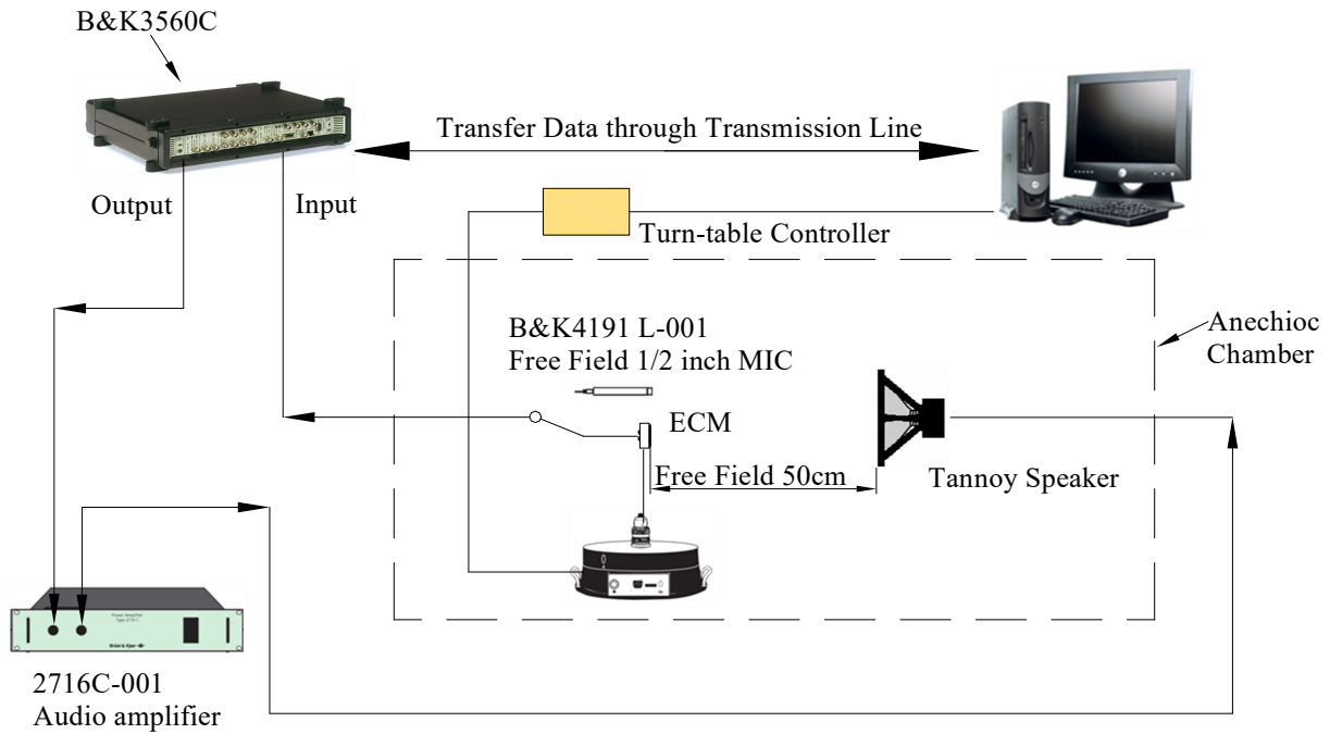
Fig. 6-1 Measurement System Setup
