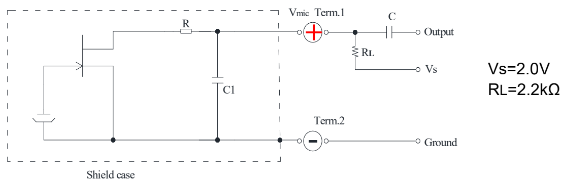
Fig. 5-1 Schematic Diagram
