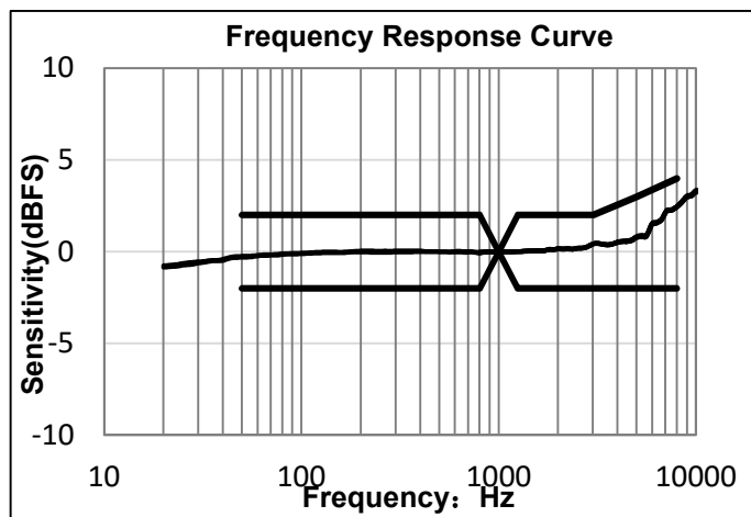
Fig. 4 Normal mode FR normalized to 1KHz
