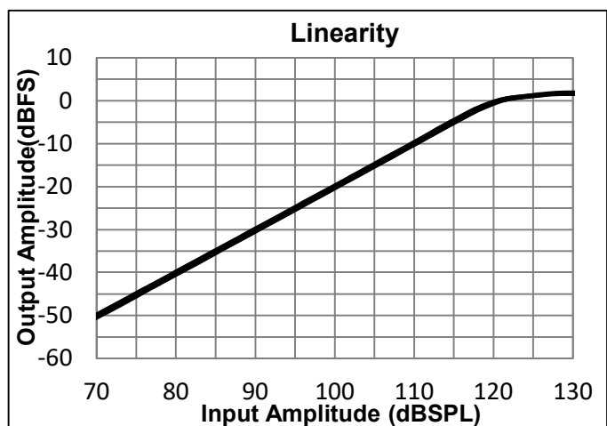
Fig. 8 Linearity
