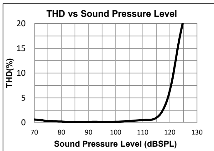
Fig. 6 Typical THD vs Sound Pressure Level
