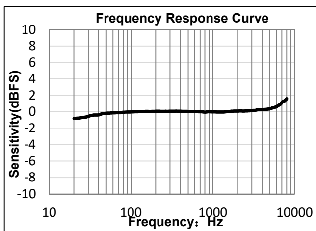
Fig. 5 Low power mode FR normalized to 1KHz
