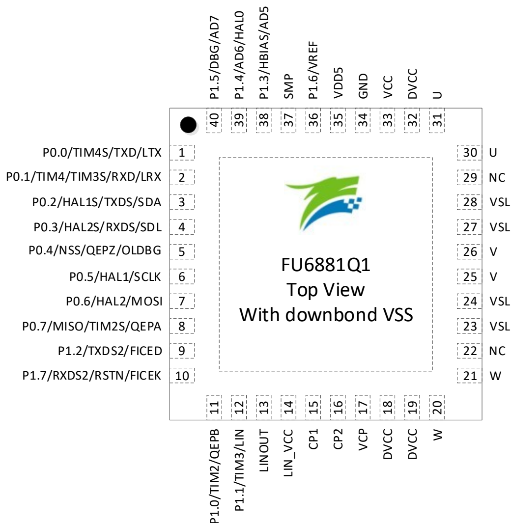
Figure 2-1 FU6881Q1 QFN40 Pinout Diagram
