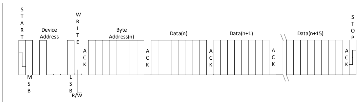
Figure 32-6 Page Write
