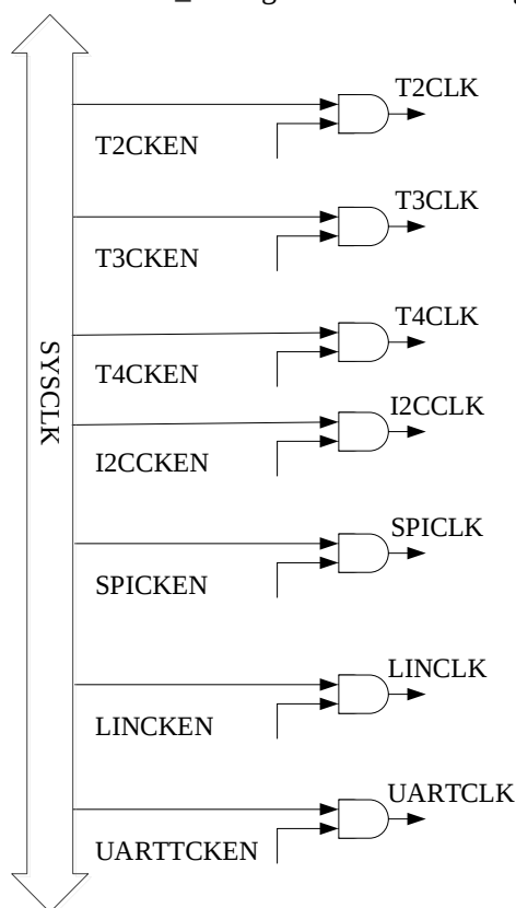
Figure 8-1 Clock Tree
