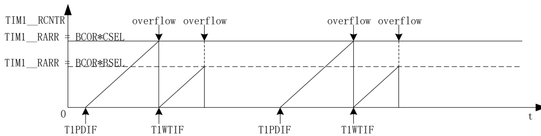
Figure 16-4 Waveform of Reload Timer
