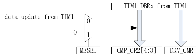
Figure 20-6 Timer1 Automatic Control of DRV_CMRR and CMP_CR2[4:3]
