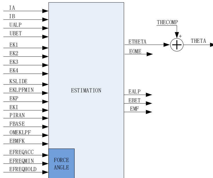
Figure 14-13 Schematic Block Diagram of Estimator
