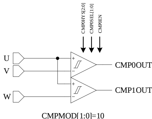
Figure 29-5 CMPG in Dual-comparator Mode
