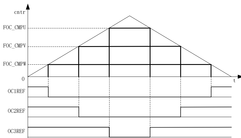
Figure 20-3 PWM Generation
