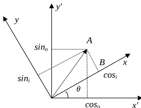
Figure 13-1 Coordinate Transformation
