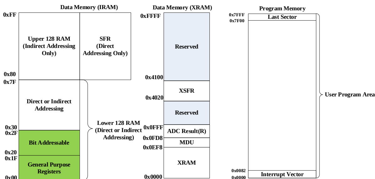
Figure 1-2 Memory Map
