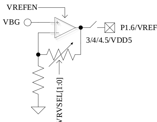
Figure 27-1 I/O Pins of VREF Module
