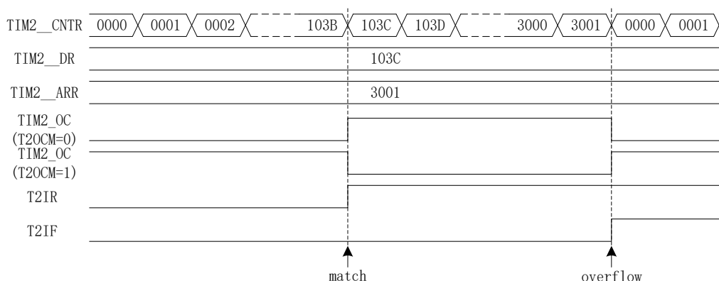
Figure 17-2 Output Mode Waveform
