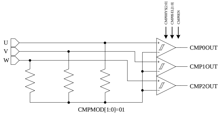
Figure 29-4 CMPG with Built-in Three Comparators and Resistors
