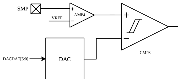
Figure 29-1 CMP3 I/O Pins
