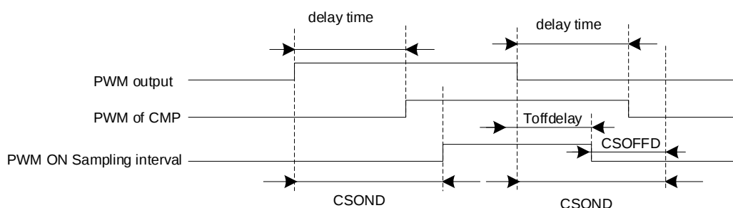
Figure 17-11 PWM ON Sampling Mode
