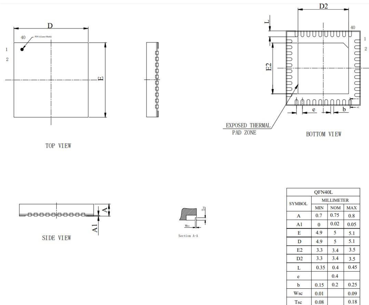
Figure 3-1 FU6881Q1 QFN40_5X5 Package Drawings and Dimensions
