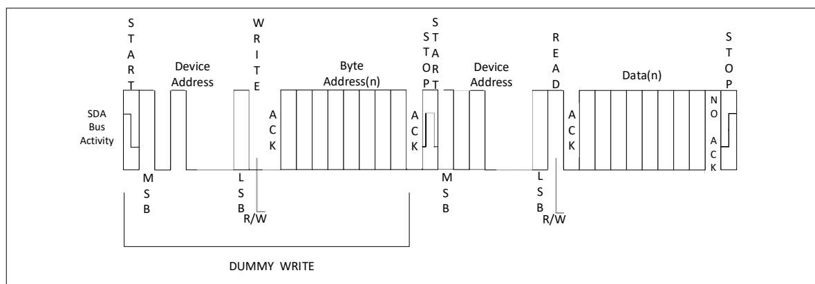
Figure 32-3 Random Read
