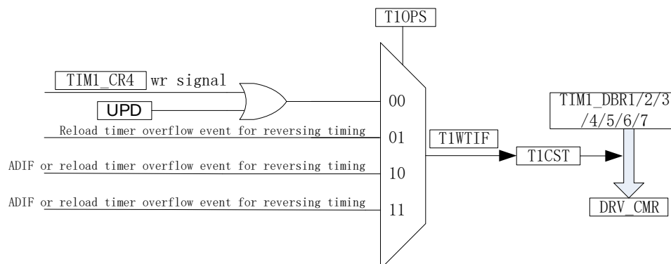
Figure 16-9 Write Timing Block Diagram
