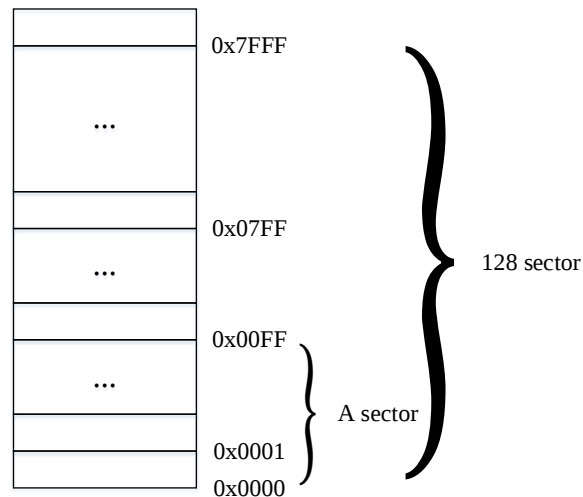
Figure 34-3 ROM Sectors
