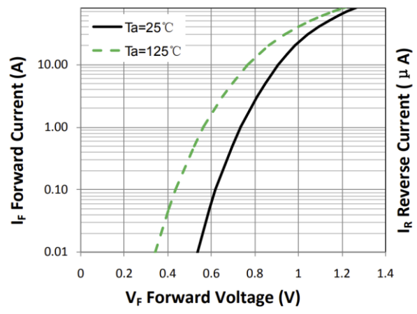
Figure 1. Forward Characteristic(typ.)
