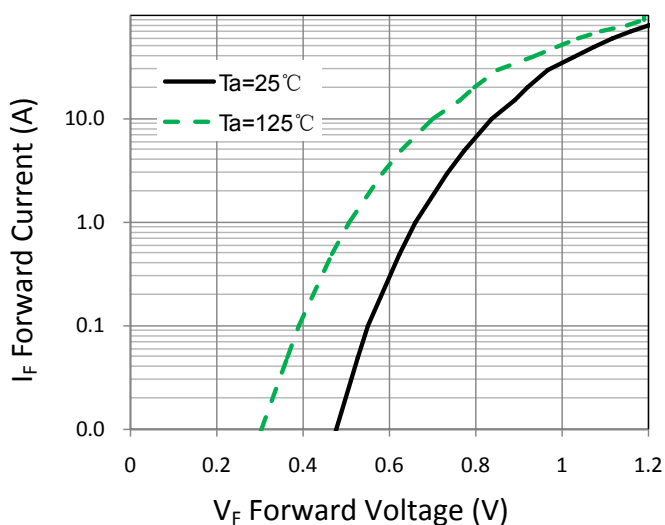
Figure 1. Forward Characteristic(typ.)
