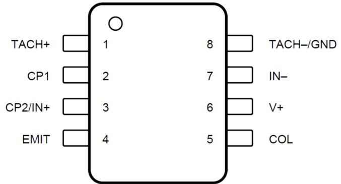
SOP-8/DIP-8
