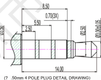
( ? .50mm 4 POLE PLUG DETAIL DRAWING )
