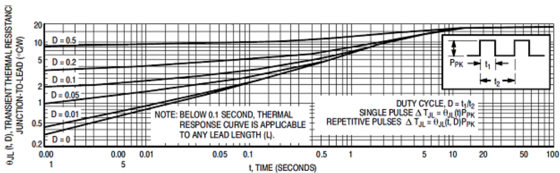
Figure 4. Typical Thermal Response L , Lead Length = 3/8 Inch
