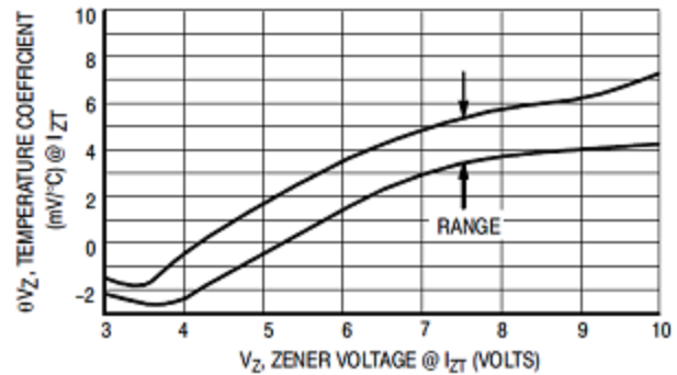
Figure 2. Temperature Coefficient-Range for Units 3 to 10 Volts
