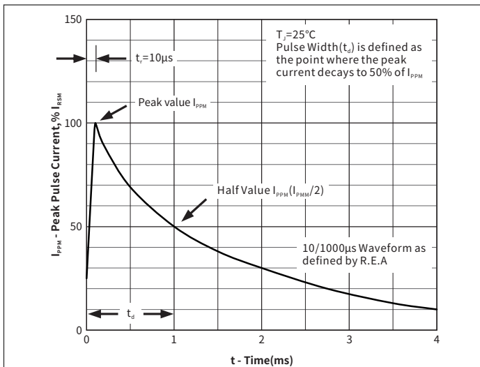
Fig.3 Pulse Waveform
