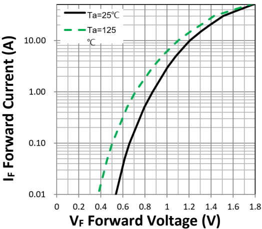
Figure 1. Forward Characteristic(typ.)
