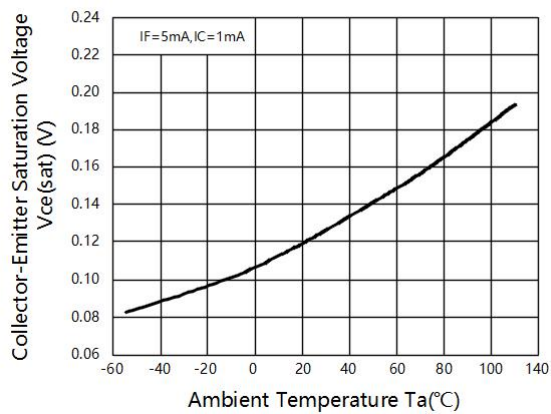
Figure9. Collector-Emitter Saturation Voltage vs Ambient Temperature T_a ( ^\circ\text{C} )
